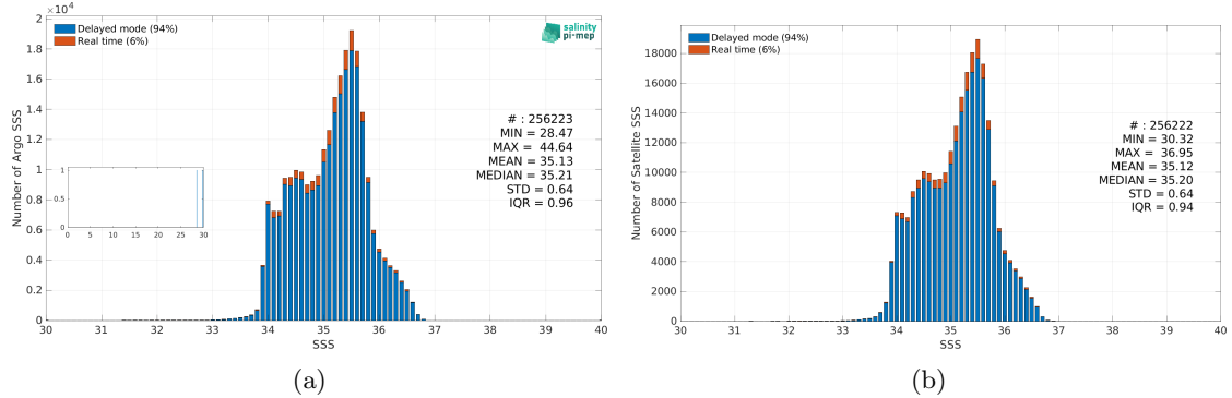
Figure 3: Histograms of SSS from Argo (a) and SMOS SSS L4 v1 - Daily (CMEMS-CNR) (b) considering all match-up pairs per bins of 0.1 over the South Pacific Ocean Pi-MEP region and for the full satellite product period.
