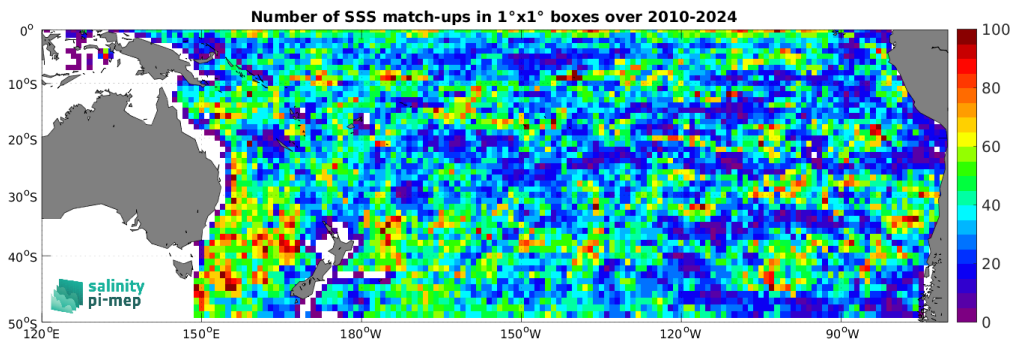
Figure 5: Number of SSS match-ups between Argo SSS and the SMOS SSS L4 v1 - Daily (CMEMS-CNR) SSS product for the South Pacific Ocean Pi-MEP region over 1^\circ \times 1^\circ boxes and for the full satellite product period.
