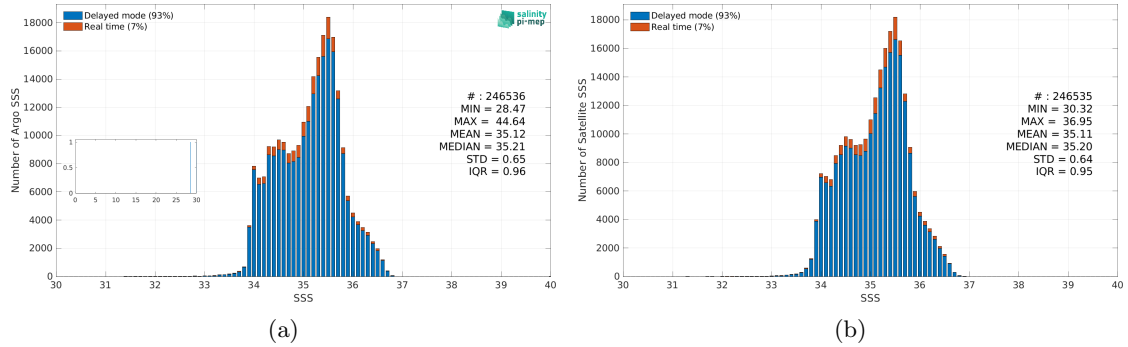
Figure 3: Histograms of SSS from Argo (a) and SMOS SSS L4 v1 - Daily (CMEMS-CNR) (b) considering all match-up pairs per bins of 0.1 over the South Pacific Ocean Pi-MEP region and for the full satellite product period.
