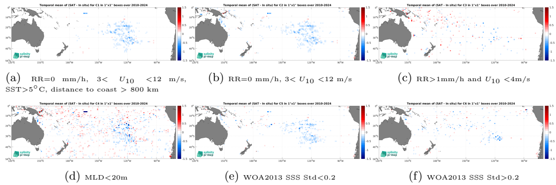
Figure 14: Temporal mean gridded over spatial boxes of size 1^\circ \times 1^\circ of \Delta SSS (SMOS SSS L4 v1 - Daily (CMEMS-CNR) - Argo) for 6 different subdatasets corresponding to:RR=0 mm/h, 3 < U_{10} < 12 m/s, SST >5^\circ\text{C} , distance to coast > 800 km (a), RR=0 mm/h, 3 < U_{10} < 12 m/s (b), RR >1 mm/h and U_{10} < 4 m/s (c),MLD <20 m (d),WOA2013 SSS Std <0.2 (e),WOA2013 SSS Std >0.2 (f).
