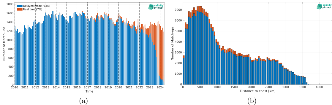
Figure 2: Number of match-ups between Argo and SMOS SSS L4 v1 - Daily (CMEMS-CNR) SSS as a function of time (a) and as function of the distance to coast (b) over the South Pacific Ocean Pi-MEP region and for the full satellite product period.
