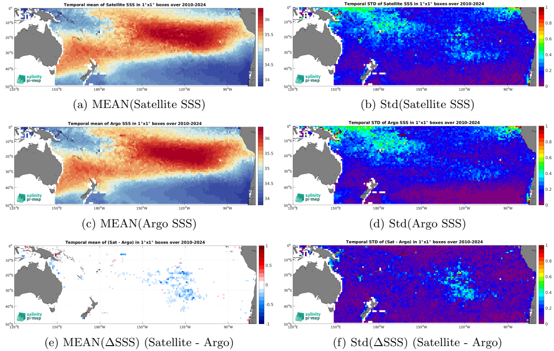
Figure 7: Temporal mean (left) and Std (right) of SSS from SMOS SSS L4 v1 - Daily (CMEMS-CNR) (top), Argo (middle), and of \Delta SSS (Satellite - Argo). Only match-up pairs are used to generate these maps.
