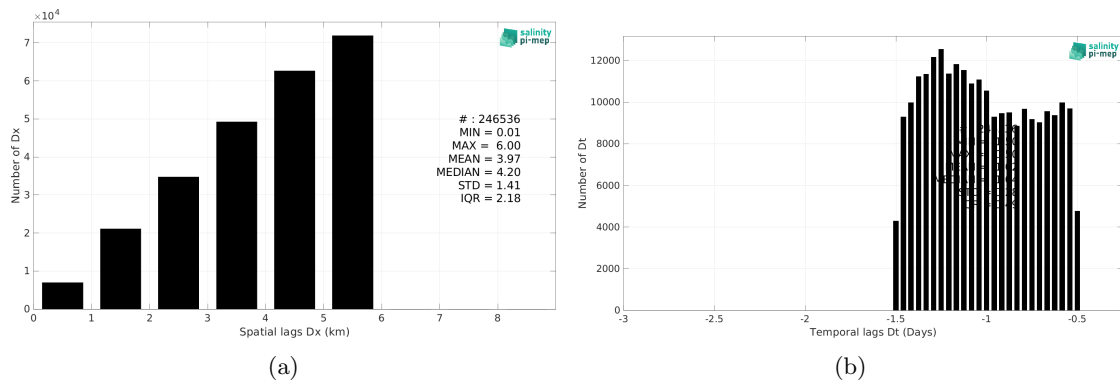
Figure 6: Histograms of the spatial (a) and temporal (b) lags between the location/time of the Argo measurement and the date of the corresponding SMOS SSS L4 v1 - Daily (CMEMS-CNR) SSS pixel.
