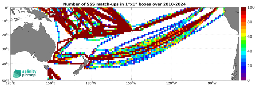
Figure 5: Number of SSS match-ups between TSG (LEGOS-DM) SSS and the SMOS SSS L4 OI v346 - Weekly (CMEMS-CATDS-LOPS) SSS product for the South Pacific Ocean Pi-MEP region over 1^\circ \times 1^\circ boxes and for the full satellite product period.
