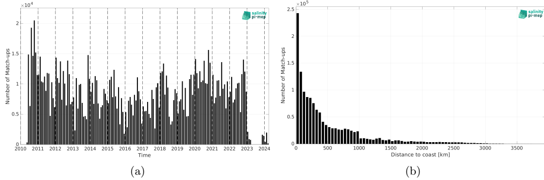
Figure 2: Number of match-ups between TSG (LEGOS-DM) and SMOS SSS L4 OI v346 - Weekly (CMEMS-CATDS-LOPS) SSS as a function of time (a) and as function of the distance to coast (b) over the South Pacific Ocean Pi-MEP region and for the full satellite product period.
