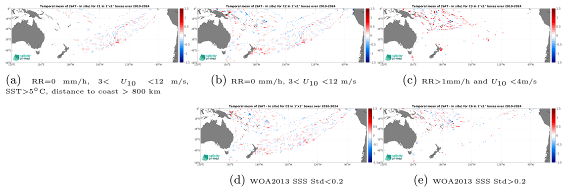
Figure 14: Temporal mean gridded over spatial boxes of size 1^\circ \times 1^\circ of \Delta SSS (SMOS SSS L4 OI v346 - Weekly (CMEMS-CATDS-LOPS) - TSG (LEGOS-DM)) for 5 different subdatasets corresponding to:RR=0 mm/h, 3 < U_{10} < 12 m/s, SST >5^\circ\text{C} , distance to coast > 800 km (a), RR=0 mm/h, 3 < U_{10} < 12 m/s (b), RR >1 mm/h and U_{10} < 4 m/s (c), WOA2013 SSS Std <0.2 (d), WOA2013 SSS Std >0.2 (e).
