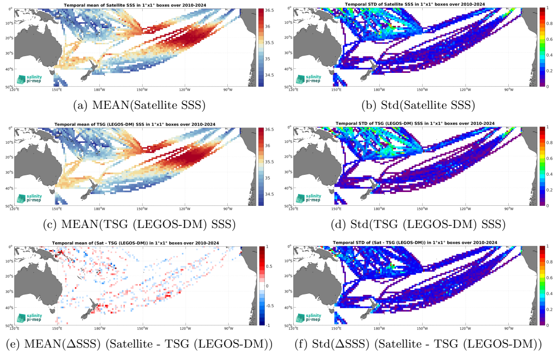
Figure 7: Temporal mean (left) and Std (right) of SSS from SMOS SSS L4 OI v346 - Weekly (CMEMS-CATDS-LOPS) (top), TSG (LEGOS-DM) (middle), and of \Delta SSS (Satellite - TSG (LEGOS-DM)). Only match-up pairs are used to generate these maps.
