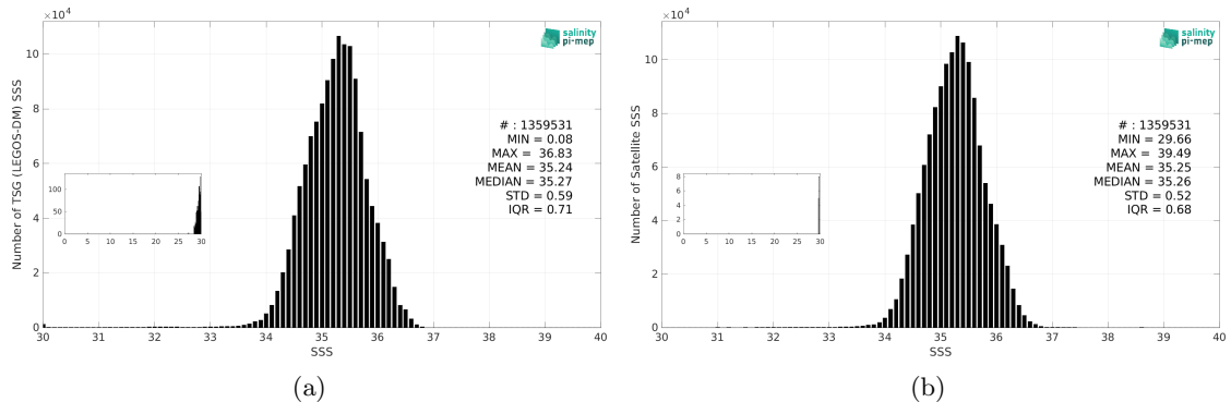
Figure 3: Histograms of SSS from TSG (LEGOS-DM) (a) and SMOS SSS L4 OI v346 - Weekly (CMEMS-CATDS-LOPS) (b) considering all match-up pairs per bins of 0.1 over the South Pacific Ocean Pi-MEP region and for the full satellite product period.
