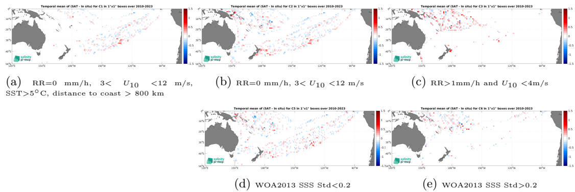
Figure 14: Temporal mean gridded over spatial boxes of size 1^\circ \times 1^\circ of \Delta\text{SSS} (SMOS SSS L4 OI v346 - Weekly (CMEMS-CATDS-LOPS) - TSG (LEGOS-DM)) for 5 different subdatasets corresponding to:RR=0 mm/h, 3 < U_{10} < 12 m/s, SST>5°C, distance to coast > 800 km (a), RR=0 mm/h, 3 < U_{10} < 12 m/s (b), RR>1mm/h and U_{10} < 4 m/s (c), WOA2013 SSS Std<0.2 (d), WOA2013 SSS Std>0.2 (e).
