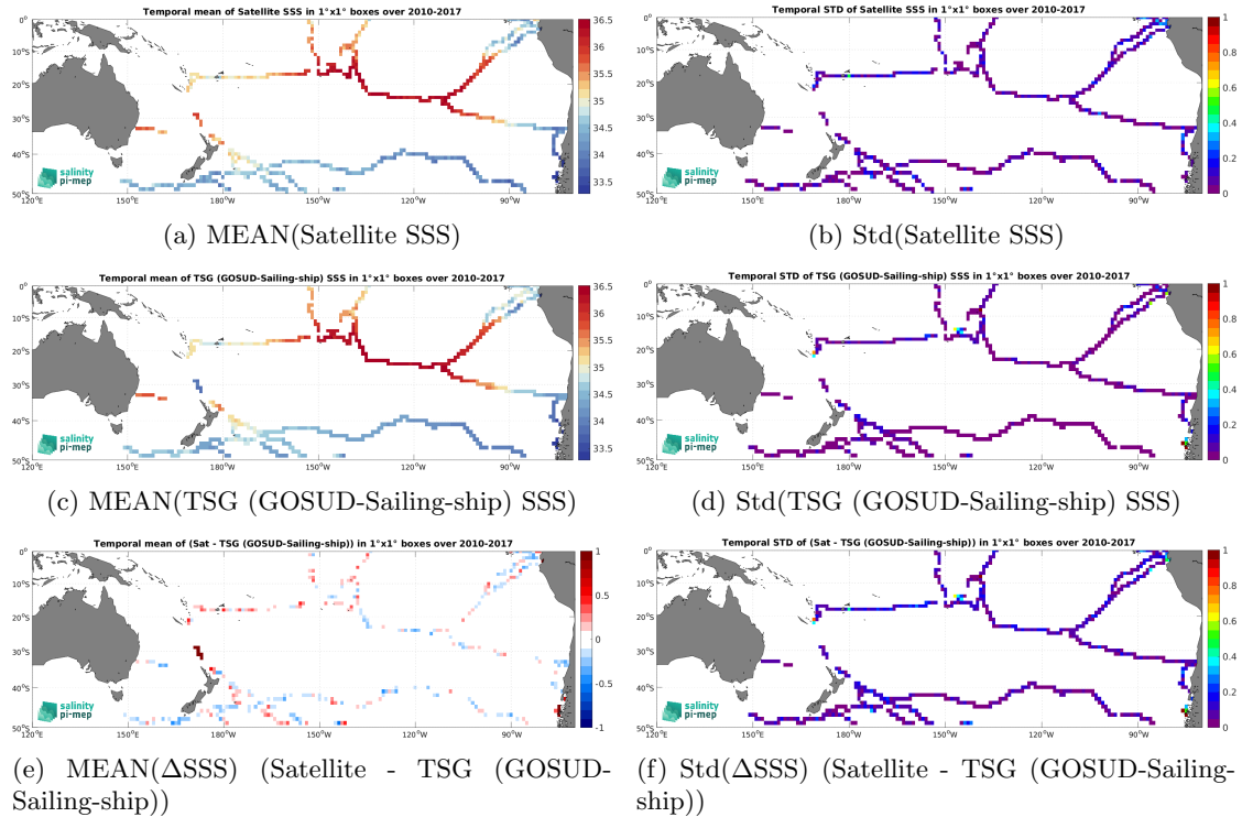
Figure 7: Temporal mean (left) and Std (right) of SSS from SMOS SSS L4 OI v346 - Weekly (CMEMS-CATDS-LOPS) (top), TSG (GOSUD-Sailing-ship) (middle), and of \Delta SSS (Satellite - TSG (GOSUD-Sailing-ship)). Only match-up pairs are used to generate these maps.
