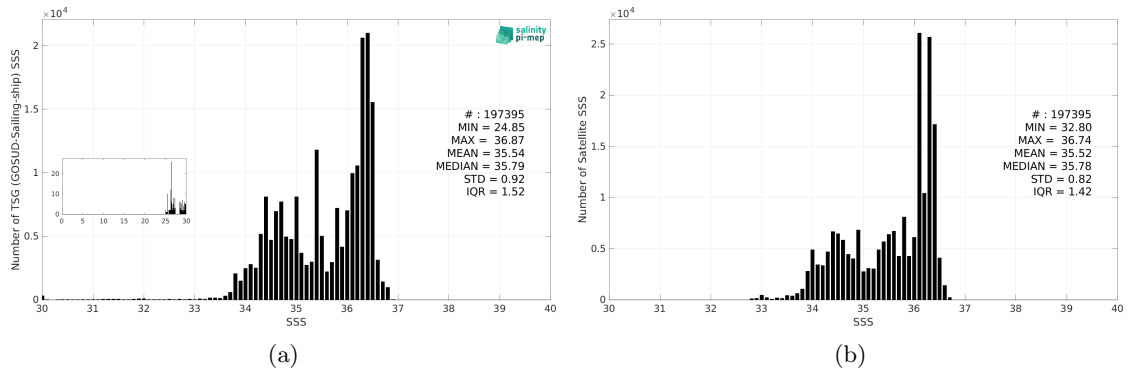
Figure 3: Histograms of SSS from TSG (GOSUD-Sailing-ship) (a) and SMOS SSS L4 OI v346 - Weekly (CMEMS-CATDS-LOPS) (b) considering all match-up pairs per bins of 0.1 over the South Pacific Ocean Pi-MEP region and for the full satellite product period.
