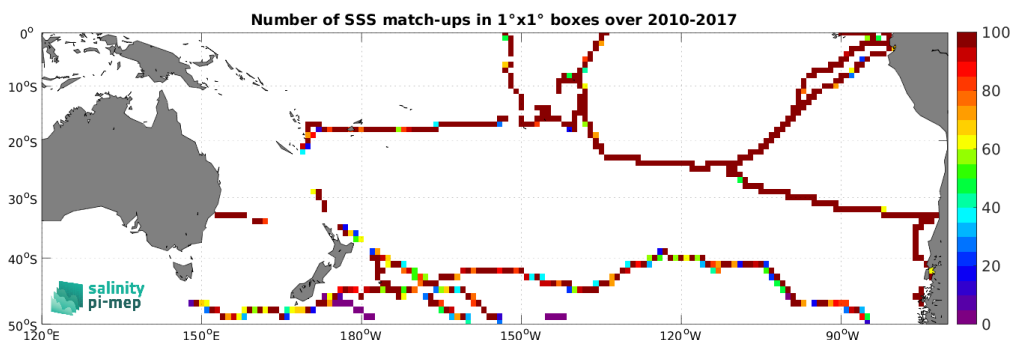
Figure 5: Number of SSS match-ups between TSG (GOSUD-Sailing-ship) SSS and the SMOS SSS L4 OI v346 - Weekly (CMEMS-CATDS-LOPS) SSS product for the South Pacific Ocean Pi-MEP region over 1^\circ \times 1^\circ boxes and for the full satellite product period.
