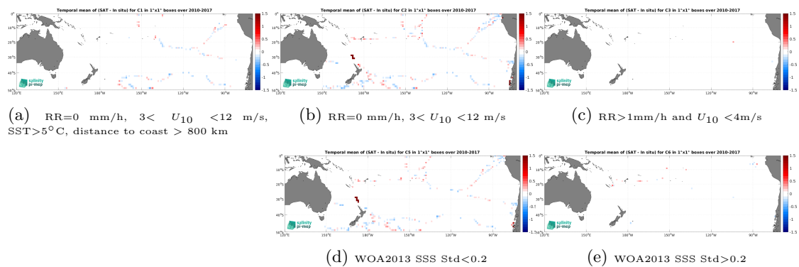
Figure 14: Temporal mean gridded over spatial boxes of size 1^\circ \times 1^\circ of \Delta SSS (SMOS SSS L4 OI v346 - Weekly (CMEMS-CATDS-LOPS) - TSG (GOSUD-Sailing-ship)) for 5 different sub-datasets corresponding to:RR=0 mm/h, 3 < U_{10} < 12 m/s, SST>5°C, distance to coast > 800 km (a), RR=0 mm/h, 3 < U_{10} < 12 m/s (b), RR>1mm/h and U_{10} < 4 m/s (c), WOA2013 SSS Std<0.2 (d), WOA2013 SSS Std>0.2 (e).
