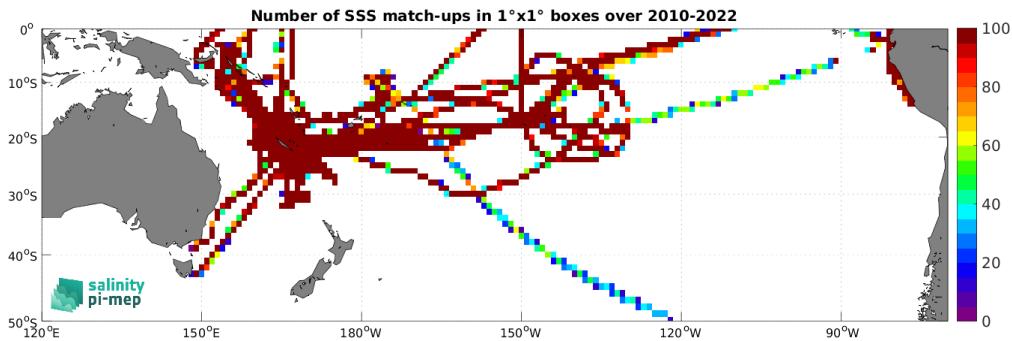
Figure 5: Number of SSS match-ups between TSG (GOSUD-Research-vessel) SSS and the SMOS SSS L4 OI v346 - Weekly (CMEMS-CATDS-LOPS) SSS product for the South Pacific Ocean Pi-MEP region over 1^\circ \times 1^\circ boxes and for the full satellite product period.
