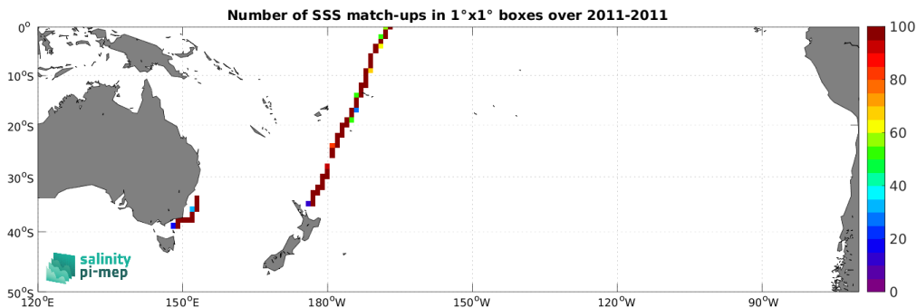
Figure 5: Number of SSS match-ups between TSG (CSIC-UTM) SSS and the SMOS SSS L4 OI v346 - Weekly (CMEMS-CATDS-LOPS) SSS product for the South Pacific Ocean Pi-MEP region over 1^\circ \times 1^\circ boxes and for the full satellite product period.
