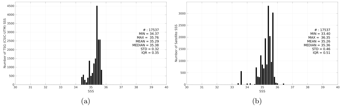
Figure 3: Histograms of SSS from TSG (CSIC-UTM) (a) and SMOS SSS L4 OI v346 - Weekly (CMEMS-CATDS-LOPS) (b) considering all match-up pairs per bins of 0.1 over the South Pacific Ocean Pi-MEP region and for the full satellite product period.
