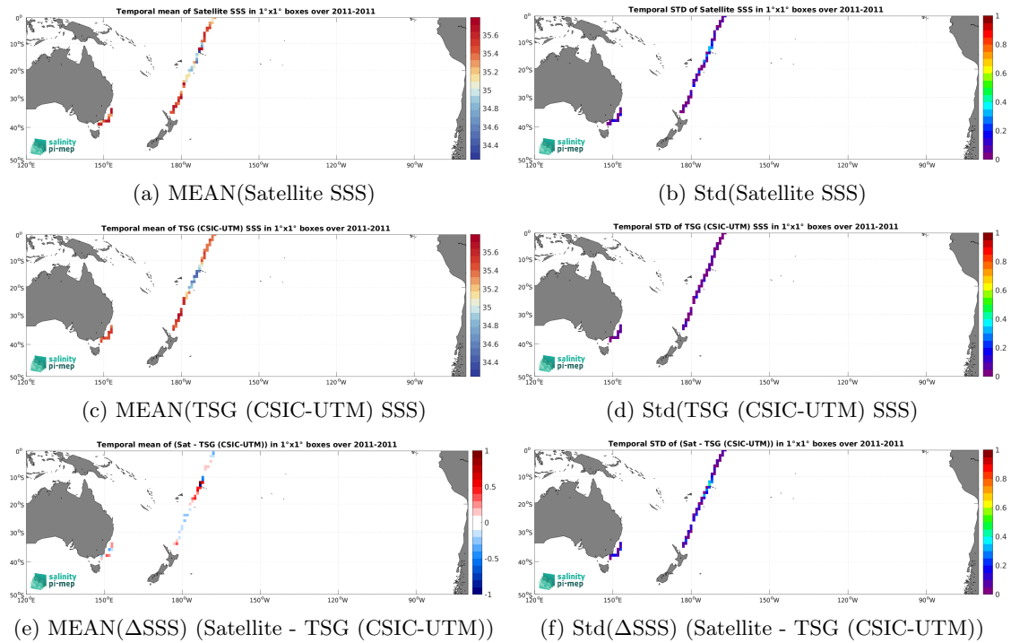
Figure 7: Temporal mean (left) and Std (right) of SSS from SMOS SSS L4 OI v346 - Weekly (CMEMS-CATDS-LOPS) (top), TSG (CSIC-UTM) (middle), and of \Delta SSS (Satellite - TSG (CSIC-UTM)). Only match-up pairs are used to generate these maps.
