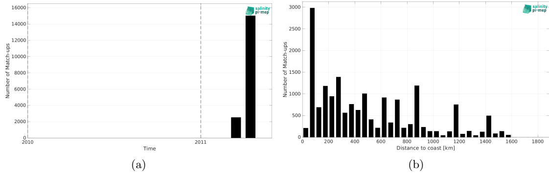
Figure 2: Number of match-ups between TSG (CSIC-UTM) and SMOS SSS L4 OI v346 - Weekly (CMEMS-CATDS-LOPS) SSS as a function of time (a) and as function of the distance to coast (b) over the South Pacific Ocean Pi-MEP region and for the full satellite product period.
