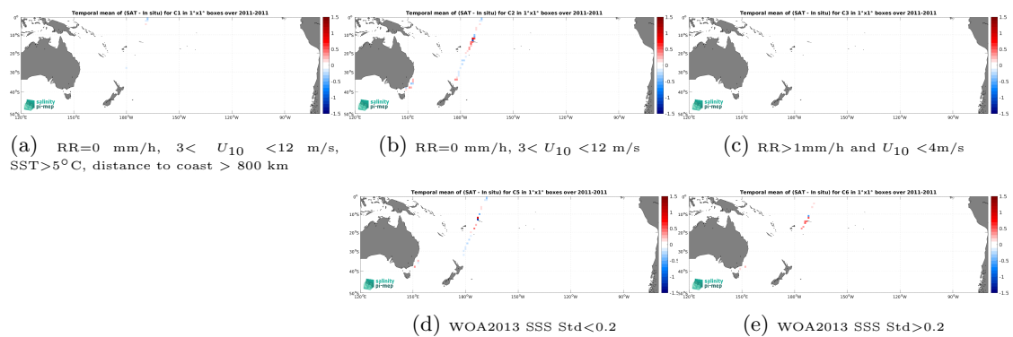
Figure 14: Temporal mean gridded over spatial boxes of size 1^\circ \times 1^\circ of \Delta SSS (SMOS SSS L4 OI v346 - Weekly (CMEMS-CATDS-LOPS) - TSG (CSIC-UTM)) for 5 different subdatasets corresponding to:RR=0 mm/h, 3 < U_{10} < 12 m/s, SST >5^\circ\text{C} , distance to coast > 800 km (a), RR=0 mm/h, 3 < U_{10} < 12 m/s (b), RR >1 mm/h and U_{10} < 4 m/s (c), WOA2013 SSS Std <0.2 (d), WOA2013 SSS Std >0.2 (e).
