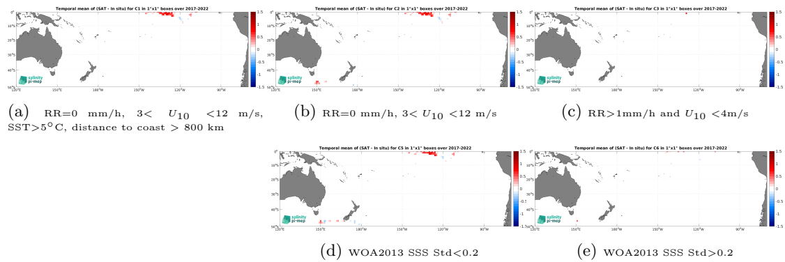
Figure 14: Temporal mean gridded over spatial boxes of size 1^\circ \times 1^\circ of \Delta\text{SSS} (SMOS SSS L4 OI v346 - Weekly (CMEMS-CATDS-LOPS) - Saildrone) for 5 different subdatasets corresponding to:RR=0 mm/h, 3 < U_{10} < 12 m/s, SST>5°C, distance to coast > 800 km (a), RR=0 mm/h, 3 < U_{10} < 12 m/s (b), RR>1mm/h and U_{10} < 4 m/s (c), WOA2013 SSS Std<0.2 (d), WOA2013 SSS Std>0.2 (e).
