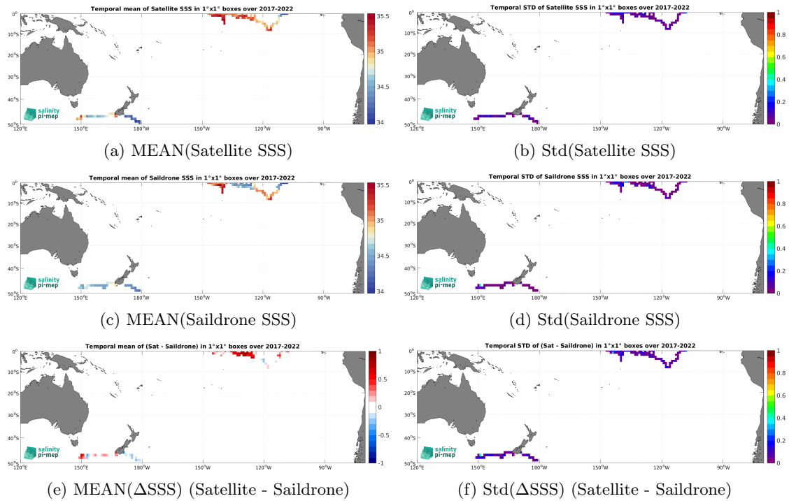
Figure 7: Temporal mean (left) and Std (right) of SSS from SMOS SSS L4 OI v346 - Weekly (CMEMS-CATDS-LOPS) (top), Saildrone (middle), and of \Delta SSS (Satellite - Saildrone). Only match-up pairs are used to generate these maps.
