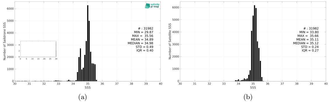
Figure 3: Histograms of SSS from Saildrone (a) and SMOS SSS L4 OI v346 - Weekly (CMEMS-CATDS-LOPS) (b) considering all match-up pairs per bins of 0.1 over the South Pacific Ocean Pi-MEP region and for the full satellite product period.
