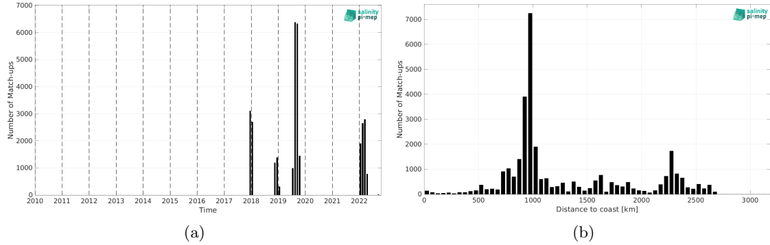
Figure 2: Number of match-ups between Saildrone and SMOS SSS L4 OI v346 - Weekly (CMEMS-CATDS-LOPS) SSS as a function of time (a) and as function of the distance to coast (b) over the South Pacific Ocean Pi-MEP region and for the full satellite product period.
