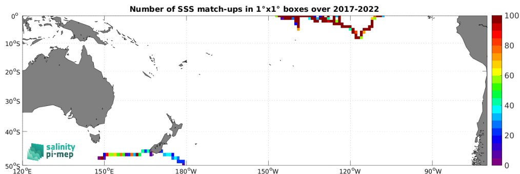
Figure 5: Number of SSS match-ups between Sairdron SSS and the SMOS SSS L4 OI v346 - Weekly (CMEMS-CATDS-LOPS) SSS product for the South Pacific Ocean Pi-MEP region over 1^\circ \times 1^\circ boxes and for the full satellite product period.
