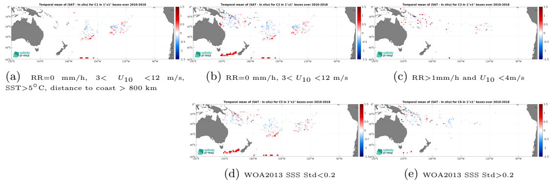
Figure 13: Temporal mean gridded over spatial boxes of size 1^\circ \times 1^\circ of \Delta SSS (SMOS SSS L4 OI v346 - Weekly (CMEMS-CATDS-LOPS) - Surface drifters) for 5 different subdatasets corresponding to:RR=0 mm/h, 3 < U_{10} < 12 m/s, SST >5^\circ C, distance to coast > 800 km (a), RR=0 mm/h, 3 < U_{10} < 12 m/s (b), RR >1 mm/h and U_{10} < 4 m/s (c), WOA2013 SSS Std <0.2 (d), WOA2013 SSS Std >0.2 (e).
