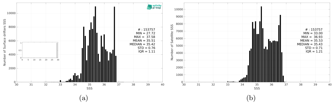
Figure 3: Histograms of SSS from Surface drifters (a) and SMOS SSS L4 OI v346 - Weekly (CMEMS-CATDS-LOPS) (b) considering all match-up pairs per bins of 0.1 over the South Pacific Ocean Pi-MEP region and for the full satellite product period.
