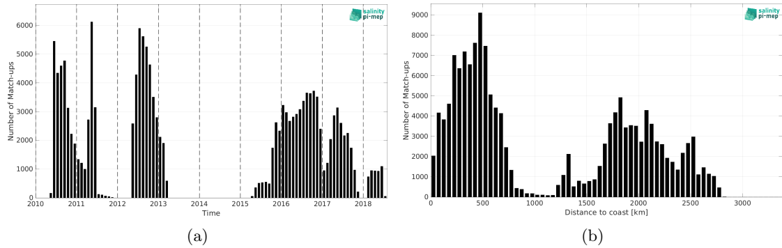
Figure 2: Number of match-ups between Surface drifters and SMOS SSS L4 OI v346 - Weekly (CMEMS-CATDS-LOPS) SSS as a function of time (a) and as function of the distance to coast (b) over the South Pacific Ocean Pi-MEP region and for the full satellite product period.
