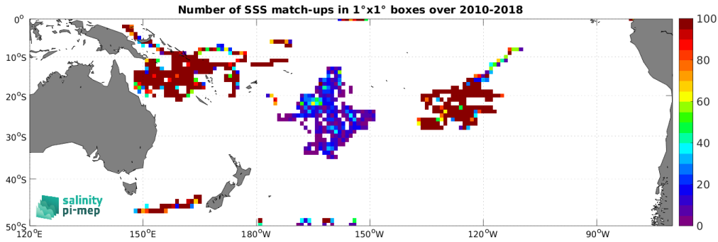
Figure 4: Number of SSS match-ups between Surface drifters SSS and the SMOS SSS L4 OI v346 - Weekly (CMEMS-CATDS-LOPS) SSS product for the South Pacific Ocean Pi-MEP region over 1^\circ \times 1^\circ boxes and for the full satellite product period.
