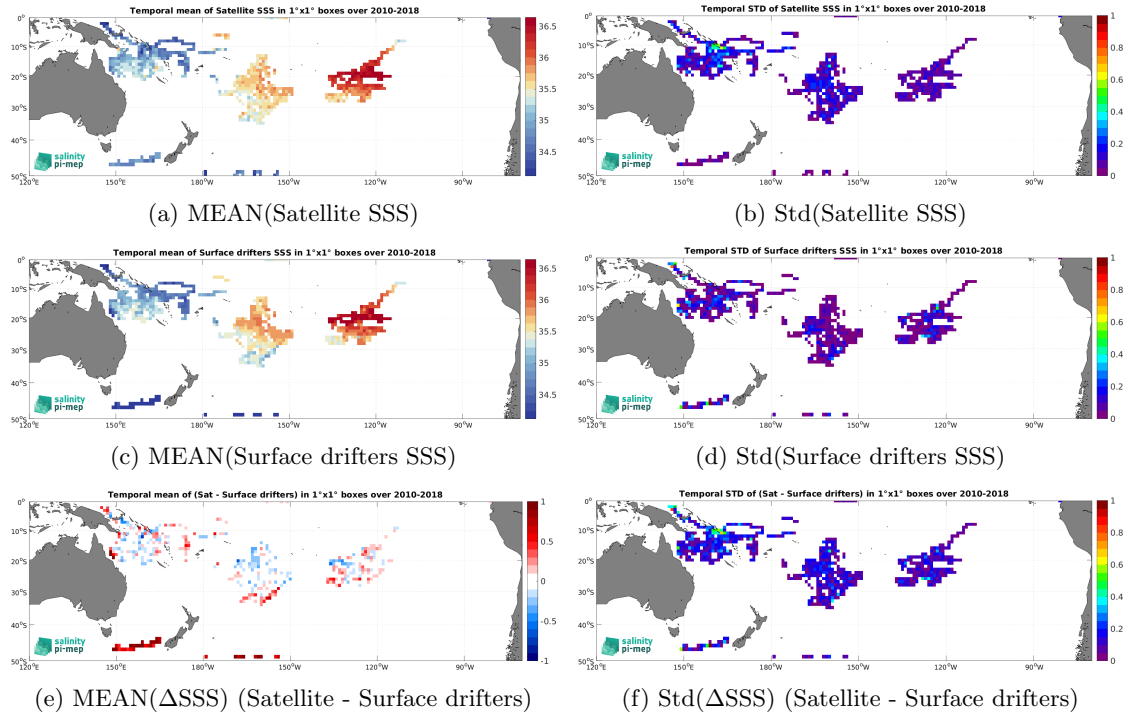
Figure 6: Temporal mean (left) and Std (right) of SSS from SMOS SSS L4 OI v346 - Weekly (CMEMS-CATDS-LOPS) (top), Surface drifters (middle), and of \Delta SSS (Satellite - Surface drifters). Only match-up pairs are used to generate these maps.
