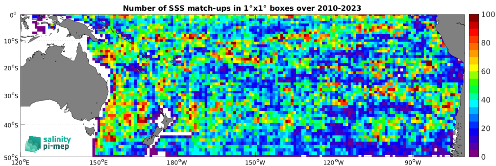
Figure 5: Number of SSS match-ups between Argo SSS and the SMOS SSS L4 OI v346 - Weekly (CMEMS-CATDS-LOPS) SSS product for the South Pacific Ocean Pi-MEP region over 1^\circ \times 1^\circ boxes and for the full satellite product period.
