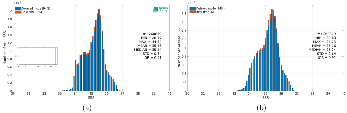
Figure 3: Histograms of SSS from Argo (a) and SMOS SSS L4 OI v346 - Weekly (CMEMS-CATDS-LOPS) (b) considering all match-up pairs per bins of 0.1 over the South Pacific Ocean Pi-MEP region and for the full satellite product period.
