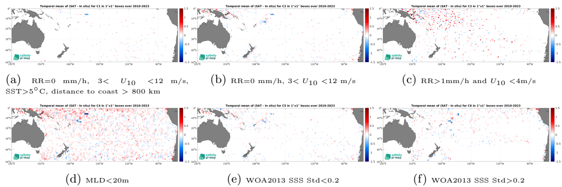
Figure 14: Temporal mean gridded over spatial boxes of size 1^\circ \times 1^\circ of \Delta SSS (SMOS SSS L4 OI v346 - Weekly (CMEMS-CATDS-LOPS) - Argo) for 6 different subdatasets corresponding to:RR=0 mm/h, 3 < U_{10} < 12 m/s, SST >5^\circ C, distance to coast > 800 km (a), RR=0 mm/h, 3 < U_{10} < 12 m/s (b), RR >1 mm/h and U_{10} < 4 m/s (c),MLD <20 m (d),WOA2013 SSS Std <0.2 (e),WOA2013 SSS Std >0.2 (f).
