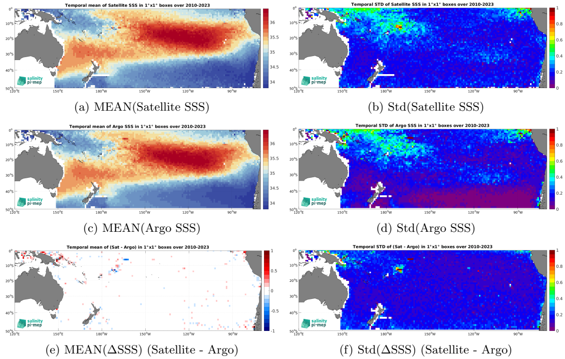
Figure 7: Temporal mean (left) and Std (right) of SSS from SMOS SSS L4 OI v346 - Weekly (CMEMS-CATDS-LOPS) (top), Argo (middle), and of \Delta SSS (Satellite - Argo). Only match-up pairs are used to generate these maps.
