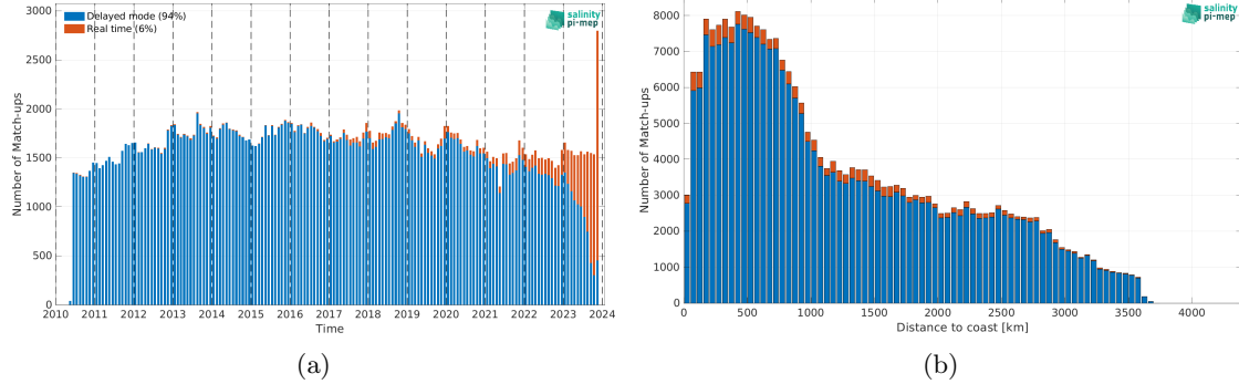
Figure 2: Number of match-ups between Argo and SMOS SSS L4 OI v346 - Weekly (CMEMS-CATDS-LOPS) SSS as a function of time (a) and as function of the distance to coast (b) over the South Pacific Ocean Pi-MEP region and for the full satellite product period.
