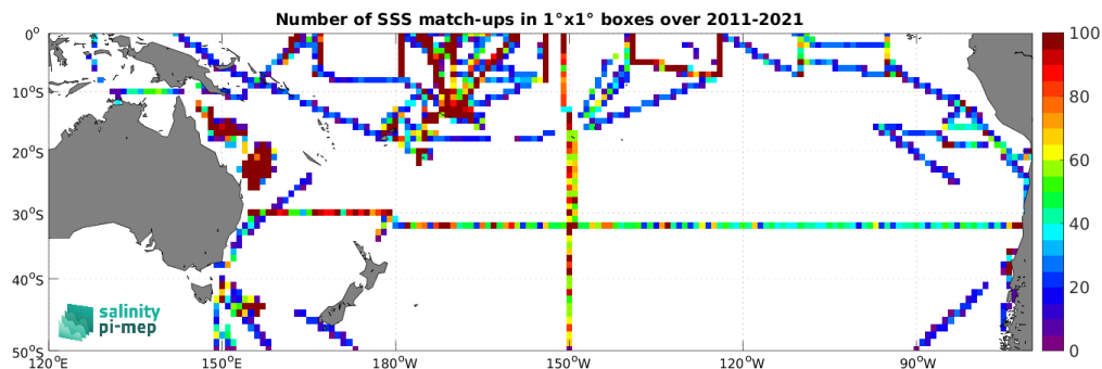
Figure 4: Number of SSS match-ups between TSG (SAMOS) SSS and the SMOS SSS L4 OI v342 - Weekly (CMEMS-CATDS-LOPS) SSS product for the South Pacific Ocean Pi-MEP region over 1^\circ \times 1^\circ boxes and for the full satellite product period.
