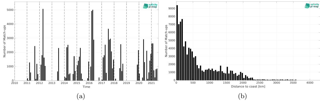
Figure 1: Number of match-ups between TSG (SAMOS) and SMOS SSS L4 OI v342 - Weekly (CMEMS-CATDS-LOPS) SSS as a function of time (a) and as function of the distance to coast (b) over the South Pacific Ocean Pi-MEP region and for the full satellite product period.
