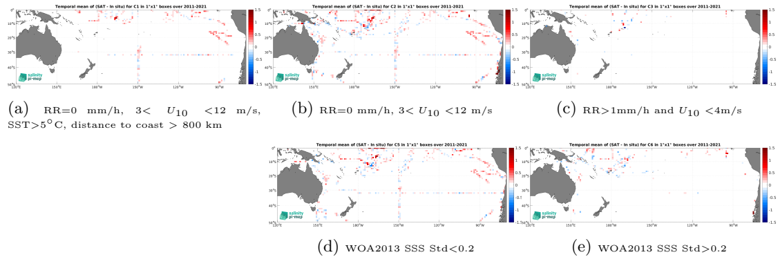
Figure 12: Temporal mean gridded over spatial boxes of size 1^\circ \times 1^\circ of \Delta SSS (SMOS SSS L4 OI v342 - Weekly (CMEMS-CATDS-LOPS) - TSG (SAMOS)) for 5 different subdatasets corresponding to:RR=0 mm/h, 3 < U_{10} < 12 m/s, SST >5^\circ C, distance to coast > 800 km (a), RR=0 mm/h, 3 < U_{10} < 12 m/s (b), RR >1 mm/h and U_{10} < 4 m/s (c), WOA2013 SSS Std <0.2 (d), WOA2013 SSS Std >0.2 (e).
