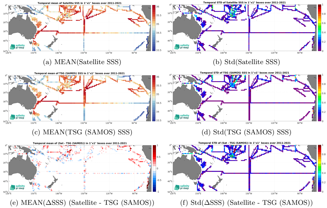
Figure 6: Temporal mean (left) and Std (right) of SSS from SMOS SSS L4 OI v342 - Weekly (CMEMS-CATDS-LOPS) (top), TSG (SAMOS) (middle), and of \Delta SSS (Satellite - TSG (SAMOS)). Only match-up pairs are used to generate these maps.
