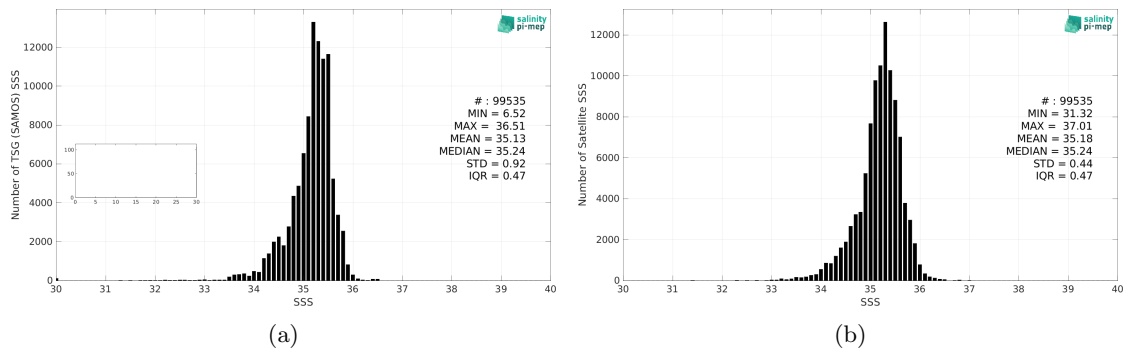
Figure 2: Histograms of SSS from TSG (SAMOS) (a) and SMOS SSS L4 OI v342 - Weekly (CMEMS-CATDS-LOPS) (b) considering all match-up pairs per bins of 0.1 over the South Pacific Ocean Pi-MEP region and for the full satellite product period.
