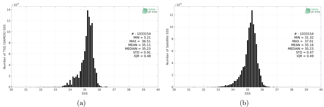
Figure 2: Histograms of SSS from TSG (SAMOS) (a) and SMOS SSS L4 OI v342 - Weekly (CMEMS-CATDS-LOPS) (b) considering all match-up pairs per bins of 0.1 over the South Pacific Ocean Pi-MEP region and for the full satellite product period.
