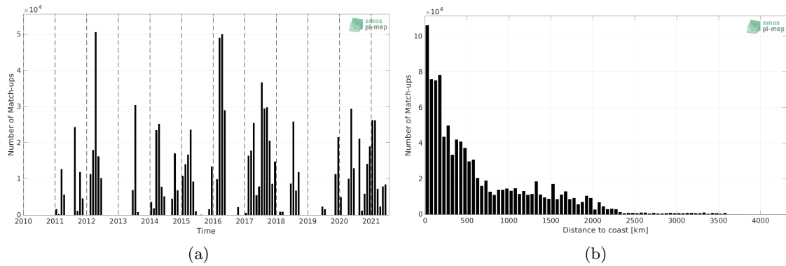
Figure 1: Number of match-ups between TSG (SAMOS) and SMOS SSS L4 OI v342 - Weekly (CMEMS-CATDS-LOPS) SSS as a function of time (a) and as function of the distance to coast (b) over the South Pacific Ocean Pi-MEP region and for the full satellite product period.
