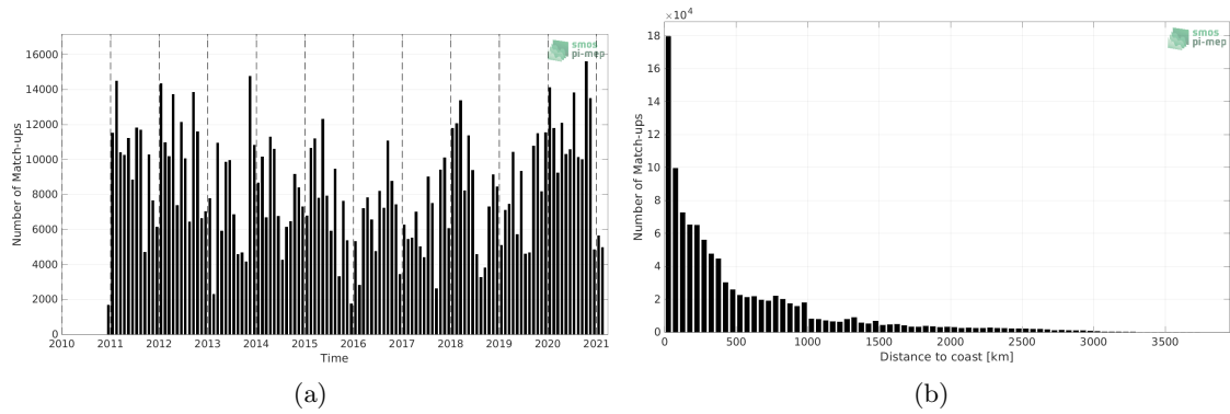
Figure 1: Number of match-ups between TSG (LEGOS-DM) and SMOS SSS L4 OI v342 - Weekly (CMEMS-CATDS-LOPS) SSS as a function of time (a) and as function of the distance to coast (b) over the South Pacific Ocean Pi-MEP region and for the full satellite product period.
