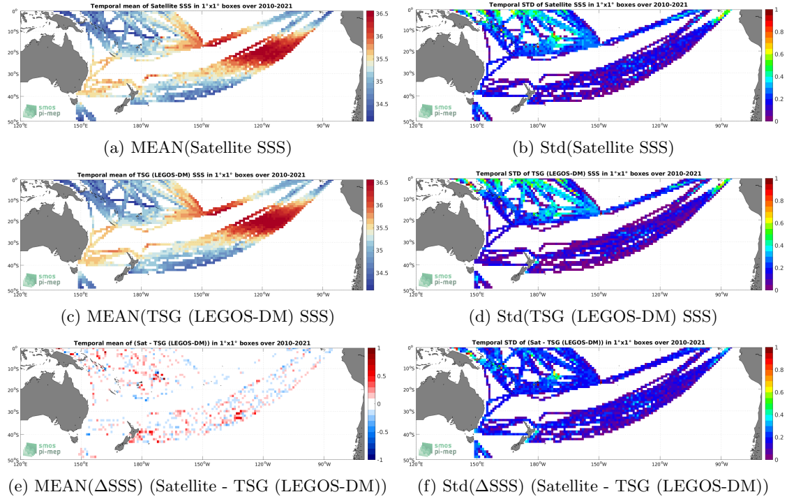
Figure 6: Temporal mean (left) and Std (right) of SSS from SMOS SSS L4 OI v342 - Weekly (CMEMS-CATDS-LOPS) (top), TSG (LEGOS-DM) (middle), and of \Delta SSS (Satellite - TSG (LEGOS-DM)). Only match-up pairs are used to generate these maps.
