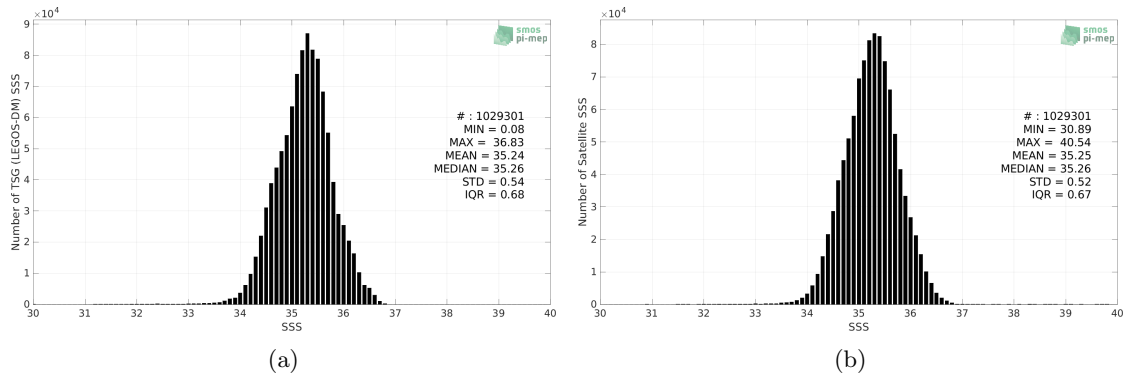
Figure 2: Histograms of SSS from TSG (LEGOS-DM) (a) and SMOS SSS L4 OI v342 - Weekly (CMEMS-CATDS-LOPS) (b) considering all match-up pairs per bins of 0.1 over the South Pacific Ocean Pi-MEP region and for the full satellite product period.
