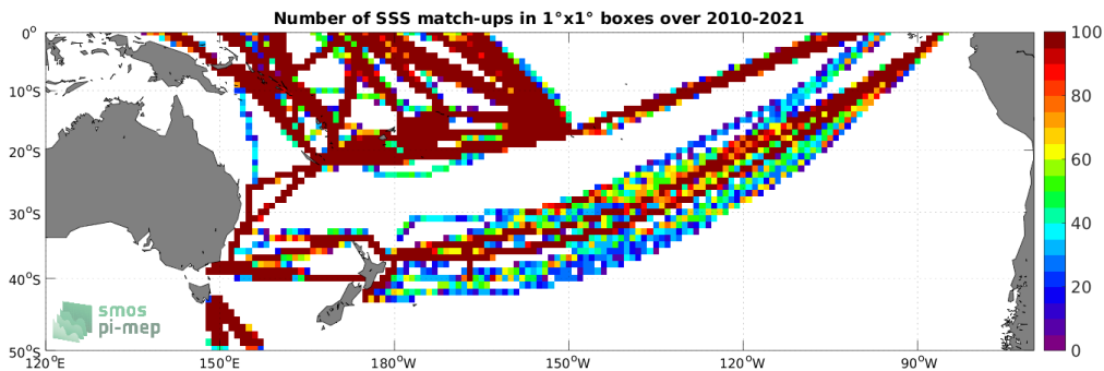
Figure 4: Number of SSS match-ups between TSG (LEGOS-DM) SSS and the SMOS SSS L4 OI v342 - Weekly (CMEMS-CATDS-LOPS) SSS product for the South Pacific Ocean Pi-MEP region over 1^\circ \times 1^\circ boxes and for the full satellite product period.
