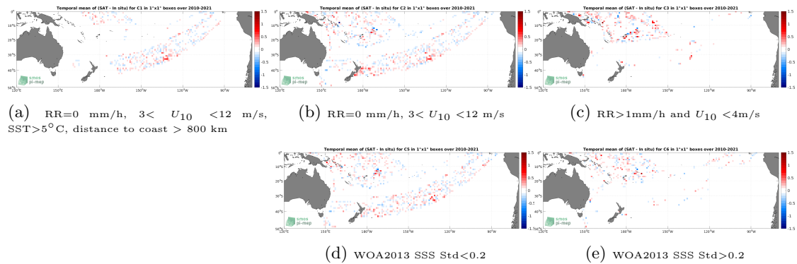
Figure 12: Temporal mean gridded over spatial boxes of size 1^\circ \times 1^\circ of \Delta SSS (SMOS SSS L4 OI v342 - Weekly (CMEMS-CATDS-LOPS) - TSG (LEGOS-DM)) for 5 different subdatasets corresponding to:RR=0 mm/h, 3 < U_{10} < 12 m/s, SST >5^\circ C, distance to coast > 800 km (a), RR=0 mm/h, 3 < U_{10} < 12 m/s (b), RR >1 mm/h and U_{10} < 4 m/s (c), WOA2013 SSS Std <0.2 (d), WOA2013 SSS Std >0.2 (e).
