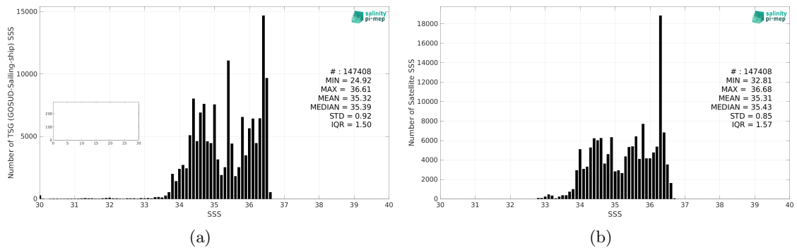
Figure 2: Histograms of SSS from TSG (GOSUD-Sailing-ship) (a) and SMOS SSS L4 OI v342 - Weekly (CMEMS-CATDS-LOPS) (b) considering all match-up pairs per bins of 0.1 over the South Pacific Ocean Pi-MEP region and for the full satellite product period.
