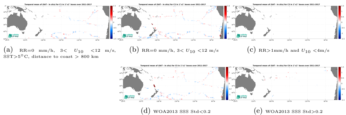
Figure 12: Temporal mean gridded over spatial boxes of size 1^\circ \times 1^\circ of \Delta SSS (SMOS SSS L4 OI v342 - Weekly (CMEMS-CATDS-LOPS) - TSG (GOSUD-Sailing-ship)) for 5 different sub-datasets corresponding to:RR=0 mm/h, 3 < U_{10} < 12 m/s, SST >5^\circ\text{C} , distance to coast > 800 km (a), RR=0 mm/h, 3 < U_{10} < 12 m/s (b), RR >1 mm/h and U_{10} < 4 m/s (c), WOA2013 SSS Std <0.2 (d), WOA2013 SSS Std >0.2 (e).
