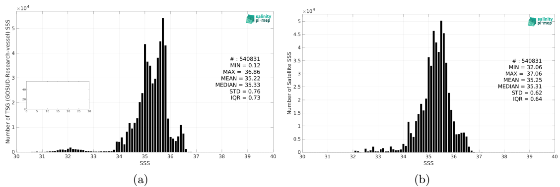
Figure 2: Histograms of SSS from TSG (GOSUD-Research-vessel) (a) and SMOS SSS L4 OI v342 - Weekly (CMEMS-CATDS-LOPS) (b) considering all match-up pairs per bins of 0.1 over the South Pacific Ocean Pi-MEP region and for the full satellite product period.
