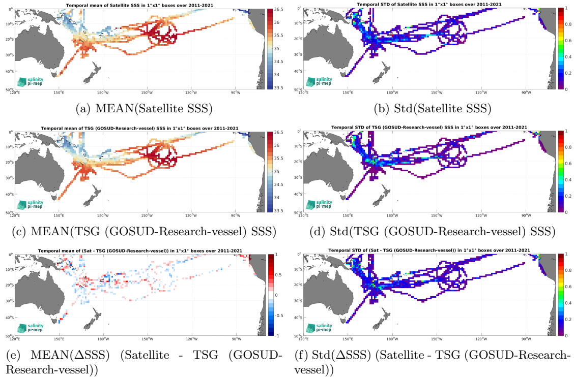
Figure 6: Temporal mean (left) and Std (right) of SSS from SMOS SSS L4 OI v342 - Weekly (CMEMS-CATDS-LOPS) (top), TSG (GOSUD-Research-vessel) (middle), and of \Delta SSS (Satellite - TSG (GOSUD-Research-vessel)). Only match-up pairs are used to generate these maps.
