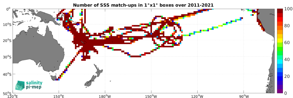
Figure 4: Number of SSS match-ups between TSG (GOSUD-Research-vessel) SSS and the SMOS SSS L4 OI v342 - Weekly (CMEMS-CATDS-LOPS) SSS product for the South Pacific Ocean Pi-MEP region over 1^\circ \times 1^\circ boxes and for the full satellite product period.
