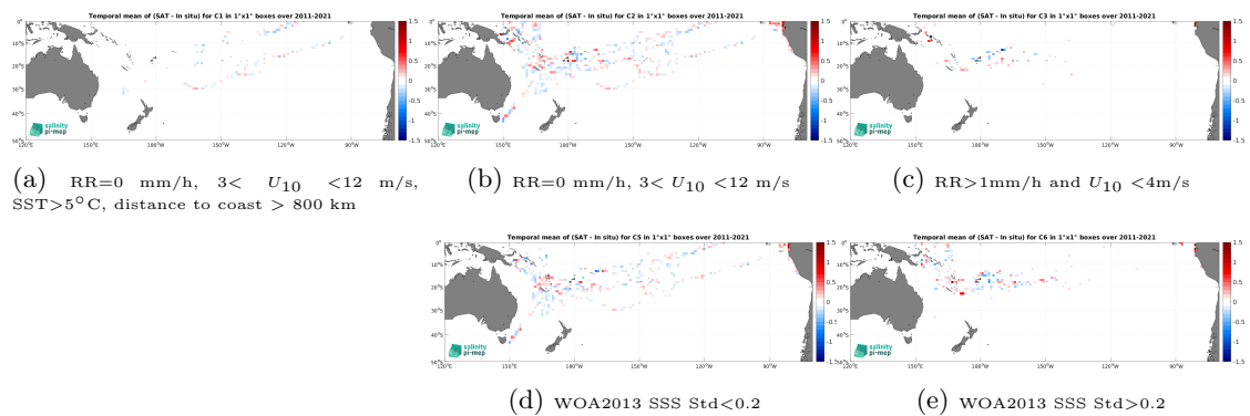
Figure 12: Temporal mean gridded over spatial boxes of size 1^\circ \times 1^\circ of \Delta SSS (SMOS SSS L4 OI v342 - Weekly (CMEMS-CATDS-LOPS) - TSG (GOSUD-Research-vessel)) for 5 different subdatasets corresponding to:RR=0 mm/h, 3 < U_{10} < 12 m/s, SST >5^\circ\text{C} , distance to coast > 800 km (a), RR=0 mm/h, 3 < U_{10} < 12 m/s (b), RR >1 mm/h and U_{10} < 4 m/s (c), WOA2013 SSS Std <0.2 (d), WOA2013 SSS Std >0.2 (e).
