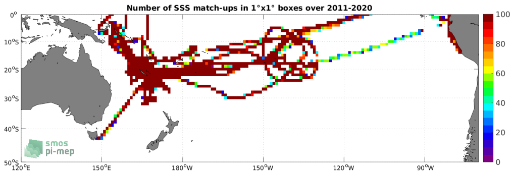
Figure 4: Number of SSS match-ups between TSG (GOSUD-Research-vessel) SSS and the SMOS SSS L4 OI v342 - Weekly (CMEMS-CATDS-LOPS) SSS product for the South Pacific Ocean Pi-MEP region over 1°×1° boxes and for the full satellite product period.
