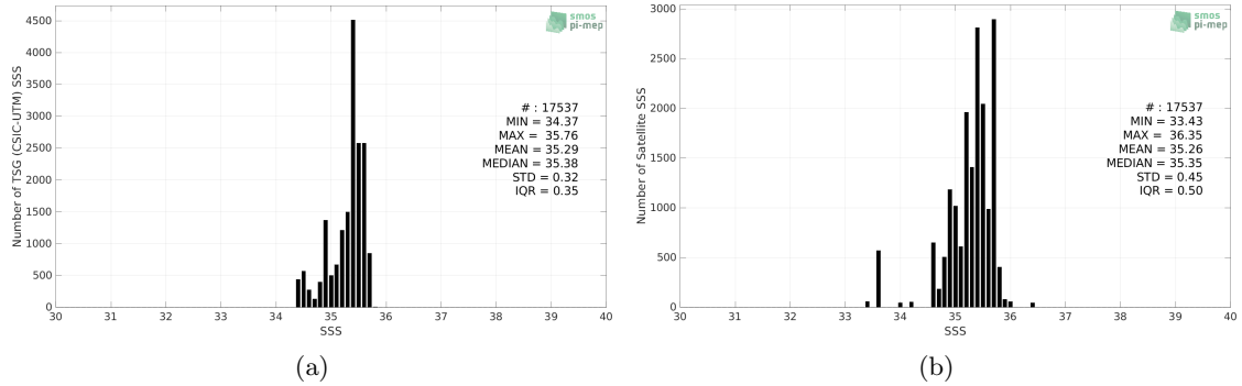
Figure 2: Histograms of SSS from TSG (CSIC-UTM) (a) and SMOS SSS L4 OI v342 - Weekly (CMEMS-CATDS-LOPS) (b) considering all match-up pairs per bins of 0.1 over the South Pacific Ocean Pi-MEP region and for the full satellite product period.
