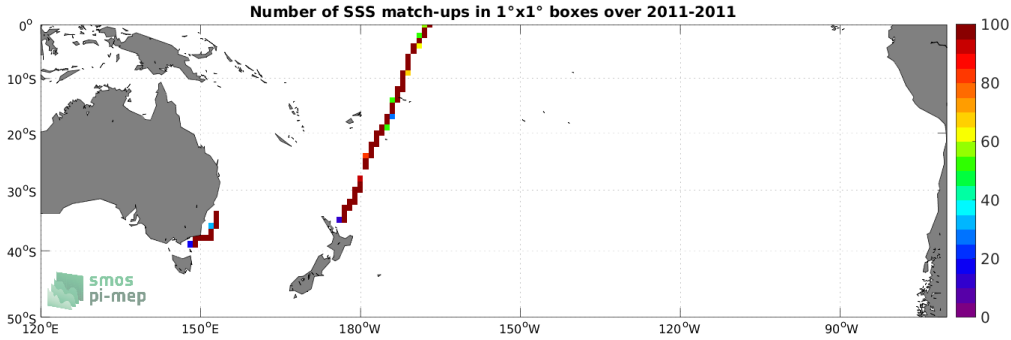
Figure 4: Number of SSS match-ups between TSG (CSIC-UTM) SSS and the SMOS SSS L4 OI v342 - Weekly (CMEMS-CATDS-LOPS) SSS product for the South Pacific Ocean Pi-MEP region over 1^\circ \times 1^\circ boxes and for the full satellite product period.
