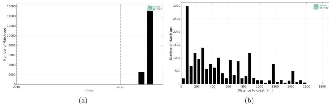
Figure 1: Number of match-ups between TSG (CSIC-UTM) and SMOS SSS L4 OI v342 - Weekly (CMEMS-CATDS-LOPS) SSS as a function of time (a) and as function of the distance to coast (b) over the South Pacific Ocean Pi-MEP region and for the full satellite product period.
