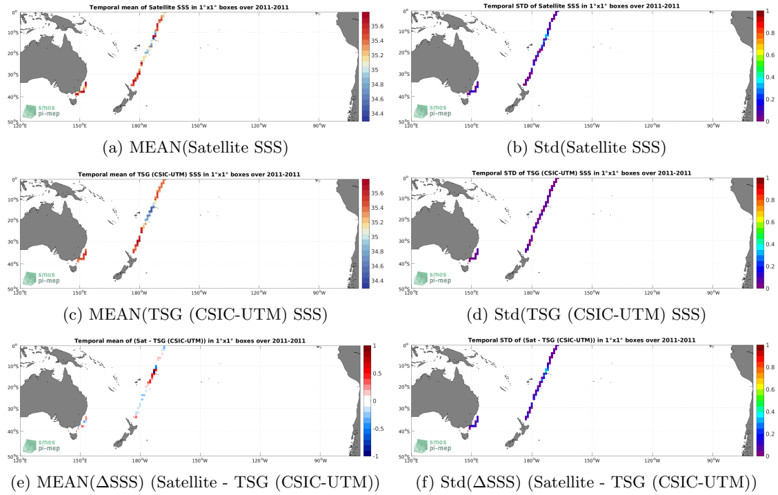
Figure 6: Temporal mean (left) and Std (right) of SSS from SMOS SSS L4 OI v342 - Weekly (CMEMS-CATDS-LOPS) (top), TSG (CSIC-UTM) (middle), and of \Delta SSS (Satellite - TSG (CSIC-UTM)). Only match-up pairs are used to generate these maps.
