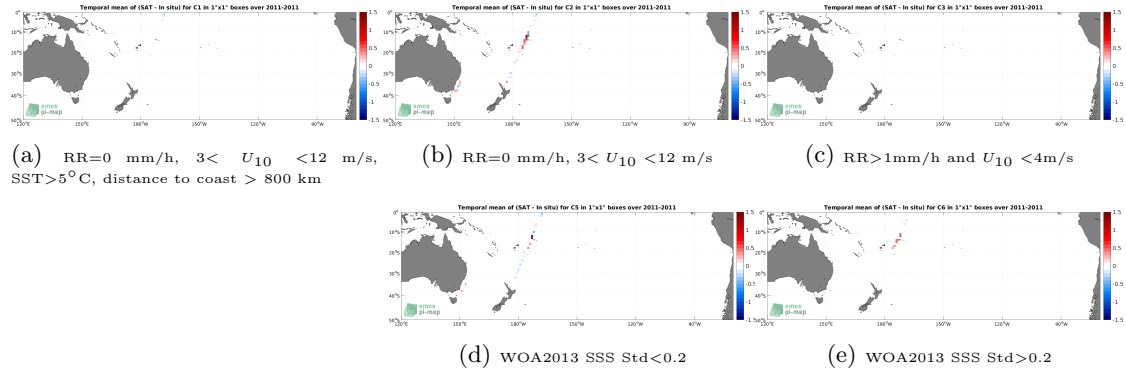
Figure 12: Temporal mean gridded over spatial boxes of size 1^{\circ}\times 1^{\circ} of \Delta\text{SSS} (SMOS SSS L4 OI v342 - Weekly (CMEMS-CATDS-LOPS) - TSG (CSIC-UTM)) for 5 different subdatasets corresponding to:RR=0 mm/h, 3 < U_{10} < 12 m/s, SST > 5^{\circ}\text{C} , distance to coast > 800 km (a), RR=0 mm/h, 3 < U_{10} < 12 m/s (b), RR > 1 mm/h and U_{10} < 4 m/s (c), WOA2013 SSS Std < 0.2 (d), WOA2013 SSS Std > 0.2 (e).
