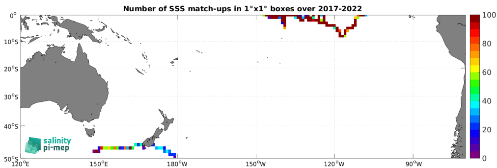
Figure 4: Number of SSS match-ups between Saildrone SSS and the SMOS SSS L4 OI v342 - Weekly (CMEMS-CATDS-LOPS) SSS product for the South Pacific Ocean Pi-MEP region over 1^\circ \times 1^\circ boxes and for the full satellite product period.
