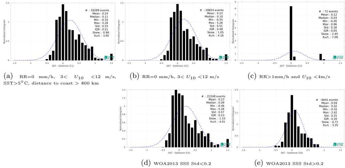
Figure 13: Normalized histogram of \Delta\text{SSS} (SMOS SSS L4 OI v342 - Weekly (CMEMS-CATDS-LOPS) - Saldrone) for 5 different subdatasets corresponding to: RR=0 mm/h, 3 < U_{10} < 12 m/s, SST>5°C, distance to coast > 800 km (a), RR=0 mm/h, 3 < U_{10} < 12 m/s (b), RR>1mm/h and U_{10} < 4 m/s (c), WOA2013 SSS Std<0.2 (d), WOA2013 SSS Std>0.2 (e).
