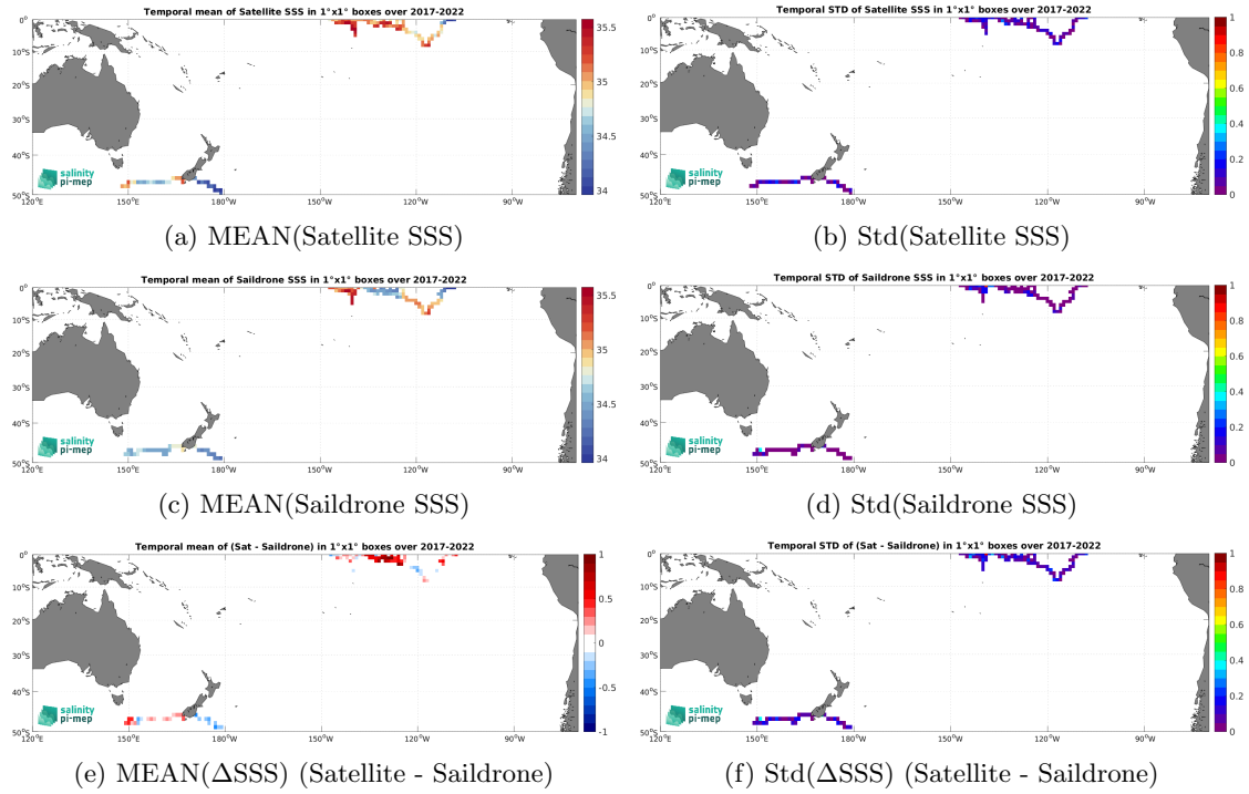
Figure 6: Temporal mean (left) and Std (right) of SSS from SMOS SSS L4 OI v342 - Weekly (CMEMS-CATDS-LOPS) (top), Saildrone (middle), and of \Delta SSS (Satellite - Saildrone). Only match-up pairs are used to generate these maps.
