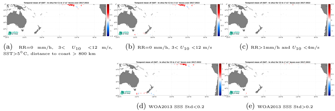
Figure 12: Temporal mean gridded over spatial boxes of size 1^\circ \times 1^\circ of \Delta SSS (SMOS SSS L4 OI v342 - Weekly (CMEMS-CATDS-LOPS) - Saildrone) for 5 different subdatasets corresponding to:RR=0 mm/h, 3 < U_{10} < 12 m/s, SST >5^\circ\text{C} , distance to coast > 800 km (a), RR=0 mm/h, 3 < U_{10} < 12 m/s (b), RR >1 mm/h and U_{10} < 4 m/s (c), WOA2013 SSS Std <0.2 (d), WOA2013 SSS Std >0.2 (e).
