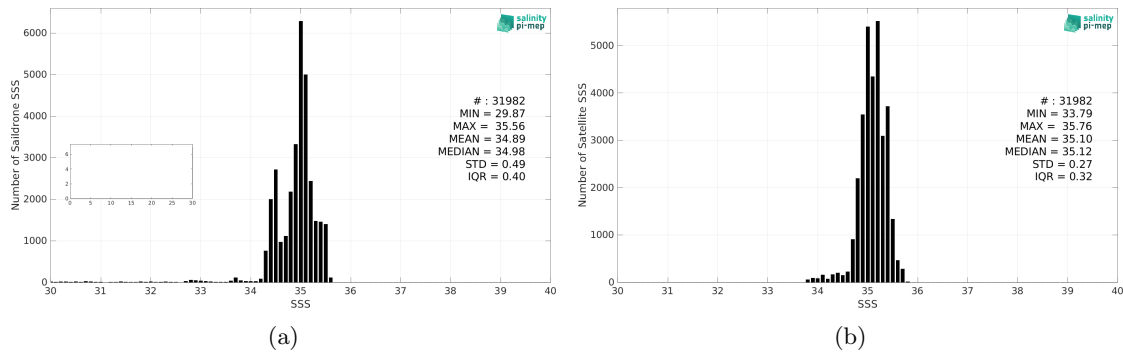
Figure 2: Histograms of SSS from Saildrone (a) and SMOS SSS L4 OI v342 - Weekly (CMEMS-CATDS-LOPS) (b) considering all match-up pairs per bins of 0.1 over the South Pacific Ocean Pi-MEP region and for the full satellite product period.
