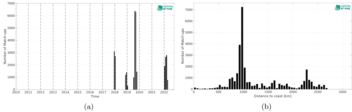
Figure 1: Number of match-ups between Saildrone and SMOS SSS L4 OI v342 - Weekly (CMEMS-CATDS-LOPS) SSS as a function of time (a) and as function of the distance to coast (b) over the South Pacific Ocean Pi-MEP region and for the full satellite product period.
