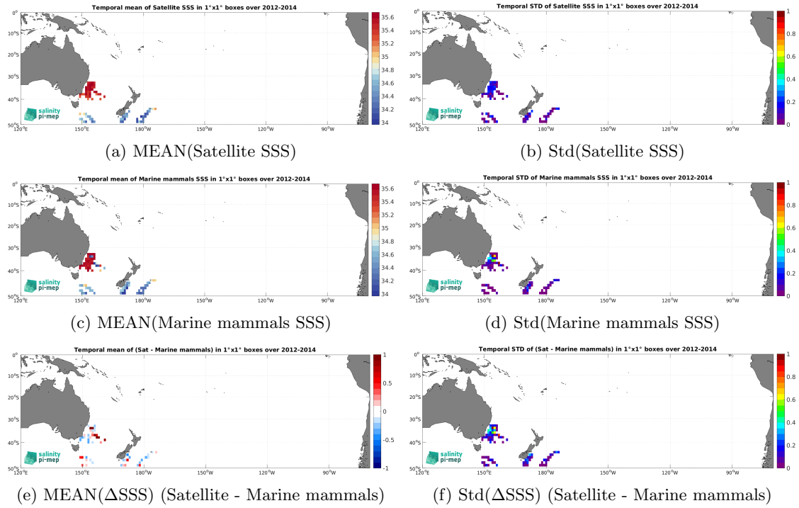
Figure 6: Temporal mean (left) and Std (right) of SSS from SMOS SSS L4 OI v342 - Weekly (CMEMS-CATDS-LOPS) (top), Marine mammals (middle), and of \Delta SSS (Satellite - Marine mammals). Only match-up pairs are used to generate these maps.
