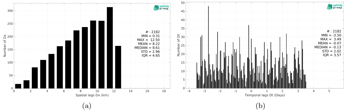
Figure 5: Histograms of the spatial (a) and temporal (b) lags between the location/time of the Marine mammals measurement and the date of the corresponding SMOS SSS L4 OI v342 - Weekly (CMEMS-CATDS-LOPS) SSS pixel.
