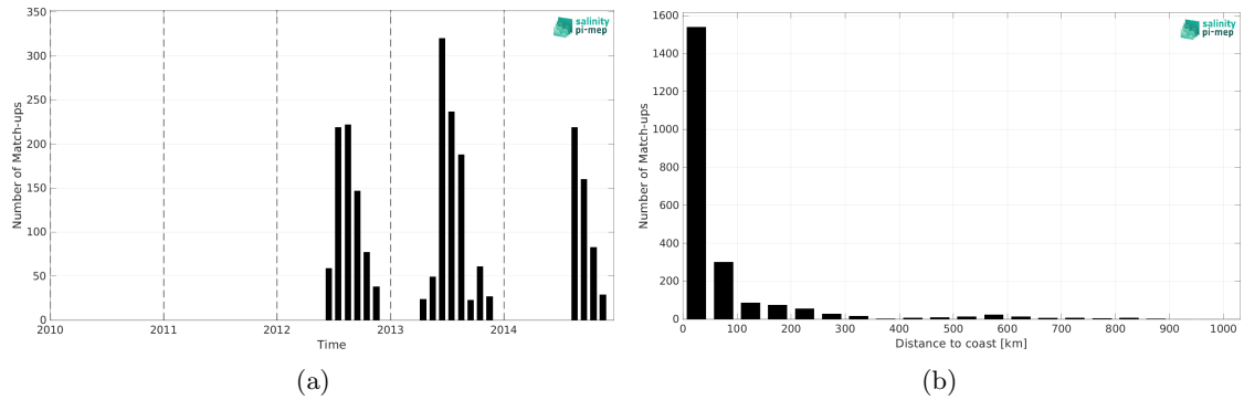
Figure 1: Number of match-ups between Marine mammals and SMOS SSS L4 OI v342 - Weekly (CMEMS-CATDS-LOPS) SSS as a function of time (a) and as function of the distance to coast (b) over the South Pacific Ocean Pi-MEP region and for the full satellite product period.
