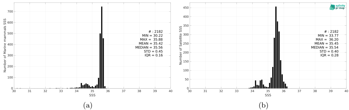
Figure 2: Histograms of SSS from Marine mammals (a) and SMOS SSS L4 OI v342 - Weekly (CMEMS-CATDS-LOPS) (b) considering all match-up pairs per bins of 0.1 over the South Pacific Ocean Pi-MEP region and for the full satellite product period.
