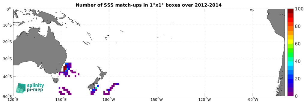
Figure 4: Number of SSS match-ups between Marine mammals SSS and the SMOS SSS L4 OI v342 - Weekly (CMEMS-CATDS-LOPS) SSS product for the South Pacific Ocean Pi-MEP region over 1^\circ \times 1^\circ boxes and for the full satellite product period.
