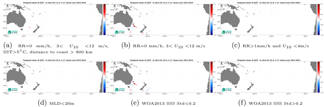
Figure 12: Temporal mean gridded over spatial boxes of size 1^{\circ}\times 1^{\circ} of \Delta\text{SSS} (SMOS SSS L4 OI v342 - Weekly (CMEMS-CATDS-LOPS) - Marine mammals) for 6 different subdatasets corresponding to:RR=0 mm/h, 3 < U_{10} < 12 m/s, SST >5^{\circ}\text{C} , distance to coast > 800 km (a), RR=0 mm/h, 3 < U_{10} < 12 m/s (b), RR >1\text{mm/h} and U_{10} < 4\text{m/s} (c),MLD <20\text{m} (d),WOA2013 SSS Std <0.2 (e),WOA2013 SSS Std >0.2 (f).
