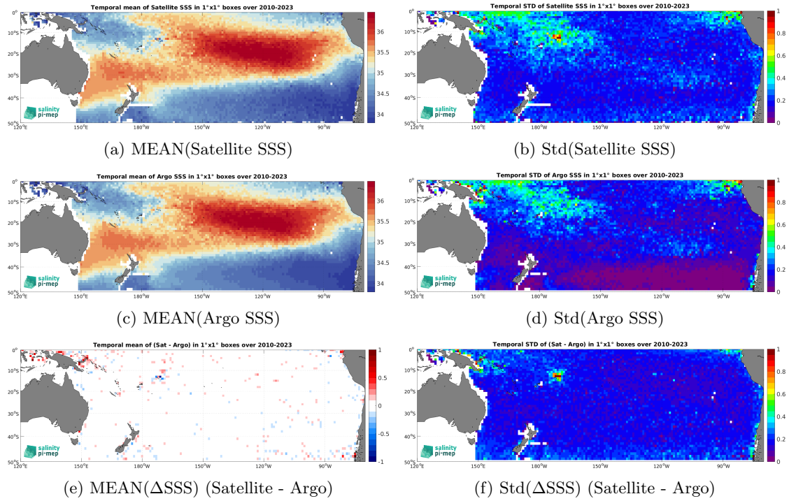
Figure 6: Temporal mean (left) and Std (right) of SSS from SMOS SSS L4 OI v342 - Weekly (CMEMS-CATDS-LOPS) (top), Argo (middle), and of \Delta SSS (Satellite - Argo). Only match-up pairs are used to generate these maps.
