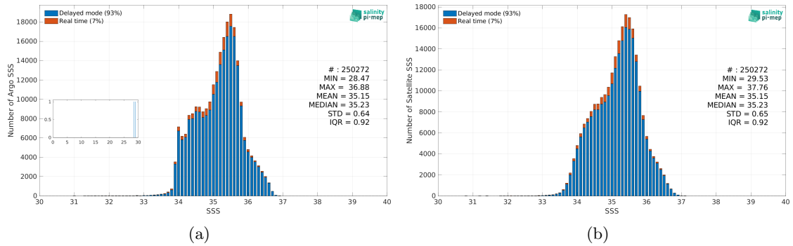
Figure 2: Histograms of SSS from Argo (a) and SMOS SSS L4 OI v342 - Weekly (CMEMS-CATDS-LOPS) (b) considering all match-up pairs per bins of 0.1 over the South Pacific Ocean Pi-MEP region and for the full satellite product period.
