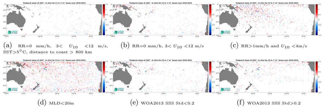
Figure 12: Temporal mean gridded over spatial boxes of size 1^\circ \times 1^\circ of \Delta SSS (SMOS SSS L4 OI v342 - Weekly (CMEMS-CATDS-LOPS) - Argo) for 6 different subdatasets corresponding to:RR=0 mm/h, 3 < U_{10} < 12 m/s, SST >5^\circ C, distance to coast > 800 km (a), RR=0 mm/h, 3 < U_{10} < 12 m/s (b), RR >1 mm/h and U_{10} < 4 m/s (c),MLD <20 m (d),WOA2013 SSS Std <0.2 (e),WOA2013 SSS Std >0.2 (f).
