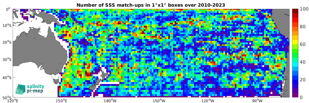
Figure 4: Number of SSS match-ups between Argo SSS and the SMOS SSS L4 OI v342 - Weekly (CMEMS-CATDS-LOPS) SSS product for the South Pacific Ocean Pi-MEP region over 1^\circ \times 1^\circ boxes and for the full satellite product period.
