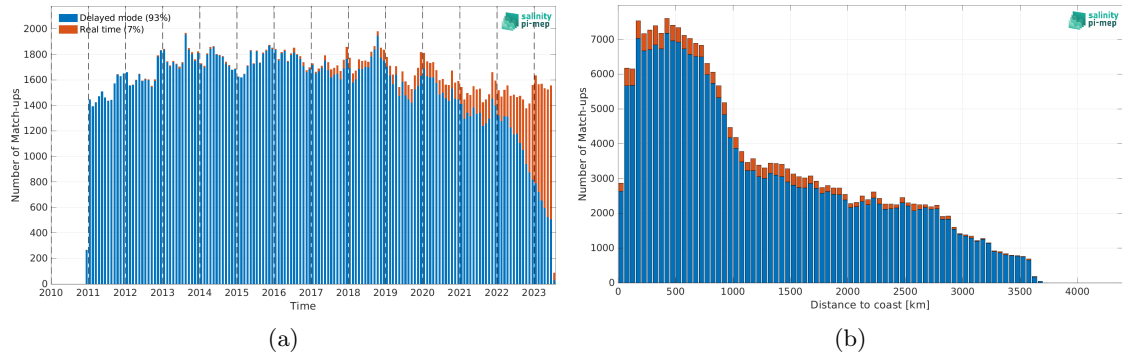
Figure 1: Number of match-ups between Argo and SMOS SSS L4 OI v342 - Weekly (CMEMS-CATDS-LOPS) SSS as a function of time (a) and as function of the distance to coast (b) over the South Pacific Ocean Pi-MEP region and for the full satellite product period.
