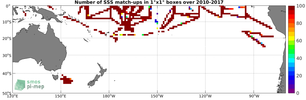
Figure 4: Number of SSS match-ups between TSG (SAMOS) SSS and the SMOS L4 v2 Weekly (CATDS-CECOS-IFREMER) SSS product for the South Pacific Ocean Pi-MEP region over 1^\circ \times 1^\circ boxes and for the full satellite product period.
