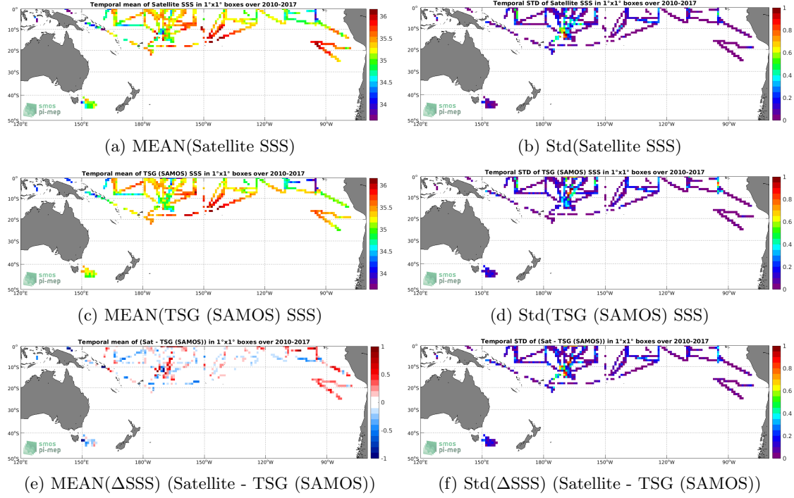
Figure 6: Temporal mean (left) and Std (right) of SSS from SMOS L4 v2 Weekly (CATDS-CECOS-IFREMER) (top), TSG (SAMOS) (middle), and of \Delta SSS (Satellite - TSG (SAMOS)). Only match-up pairs are used to generate these maps.
