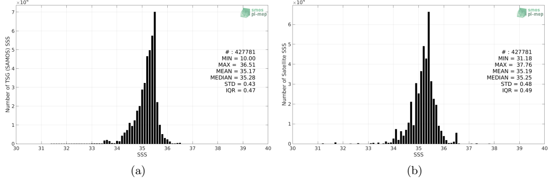
Figure 2: Histograms of SSS from TSG (SAMOS) (a) and SMOS L4 v2 Weekly (CATDS-CECOS-IFREMER) (b) considering all match-up pairs per bins of 0.1 over the South Pacific Ocean Pi-MEP region and for the full satellite product period.
