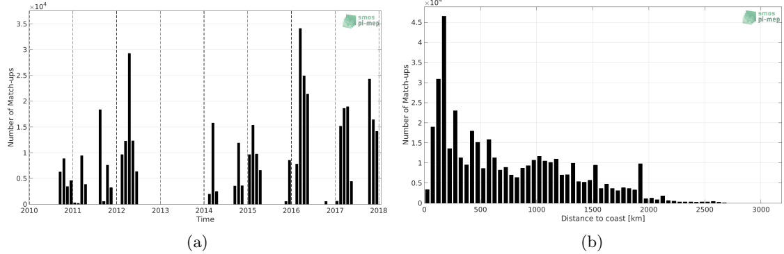
Figure 1: Number of match-ups between TSG (SAMOS) and SMOS L4 v2 Weekly (CATDS-CECOS-IFREMER) SSS as a function of time (a) and as function of the distance to coast (b) over the South Pacific Ocean Pi-MEP region and for the full satellite product period.
