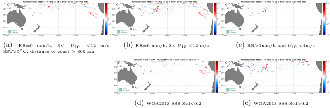
Figure 12: Temporal mean gridded over spatial boxes of size 1^\circ \times 1^\circ of \Delta SSS (SMOS L4 v2 Weekly (CATDS-CECOS-IFREMER) - TSG (SAMOS)) for 5 different subdatasets corresponding to: RR=0 mm/h, 3 < U_{10} < 12 m/s, SST > 5^\circ\text{C} , distance to coast > 800 km (a), RR=0 mm/h, 3 < U_{10} < 12 m/s (b), RR > 1 mm/h and U_{10} < 4 m/s (c), WOA2013 SSS Std < 0.2 (d), WOA2013 SSS Std > 0.2 (e).
