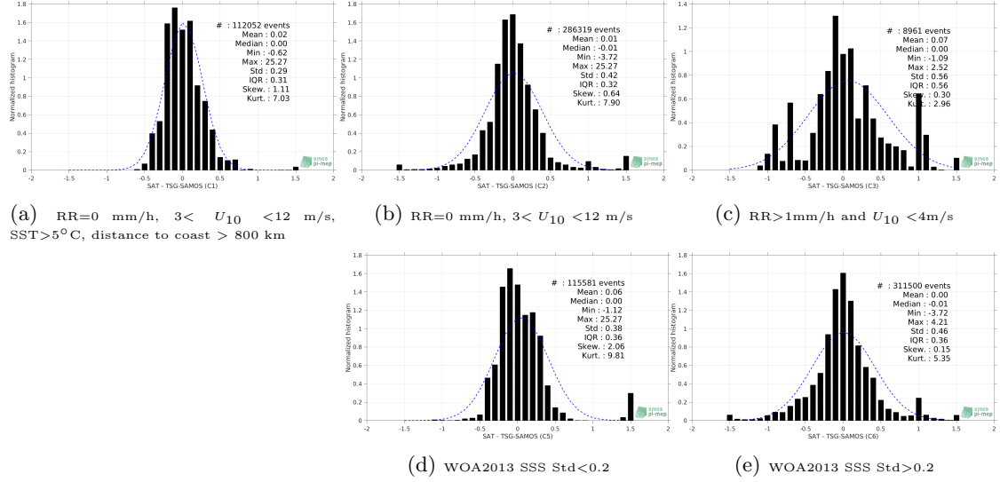
Figure 13: Normalized histogram of \Delta\text{SSS} (SMOS-L4-CATDS-CECOS-IFREMER-V2-WEEKLY-0.5DEG - TSG-SAMOS) for 5 different subdatasets corresponding to: RR=0 mm/h, 3 < U_{10} < 12 m/s, SST > 5^{\circ}\text{C} , distance to coast > 800 km (a), RR=0 mm/h, 3 < U_{10} < 12 m/s (b), RR > 1\text{mm/h} and U_{10} < 4\text{m/s} (c), WOA2013 SSS Std < 0.2 (d), WOA2013 SSS Std > 0.2 (e).
