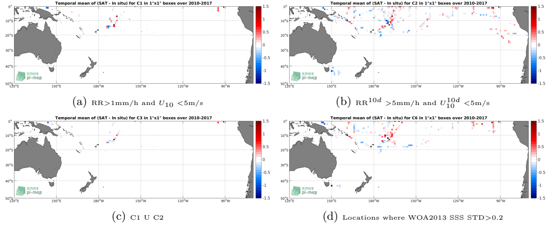
Figure 12: Temporal mean gridded over spatial boxes of size 1^\circ \times 1^\circ of \Delta SSS (SMOS-L4-CATDS-CECOS-IFREMER-V2-WEEKLY-0.5DEG - TSG-SAMOS) for 4 different subdatasets corresponding to: RR > 1\text{mm/h} and U_{10} < 5\text{m/s} (a), RR^{10d} > 5\text{mm/h} and U_{10}^{10d} < 5\text{m/s} (b), C1 U C2 (c), Locations where WOA2013 SSS STD > 0.2 (d).
