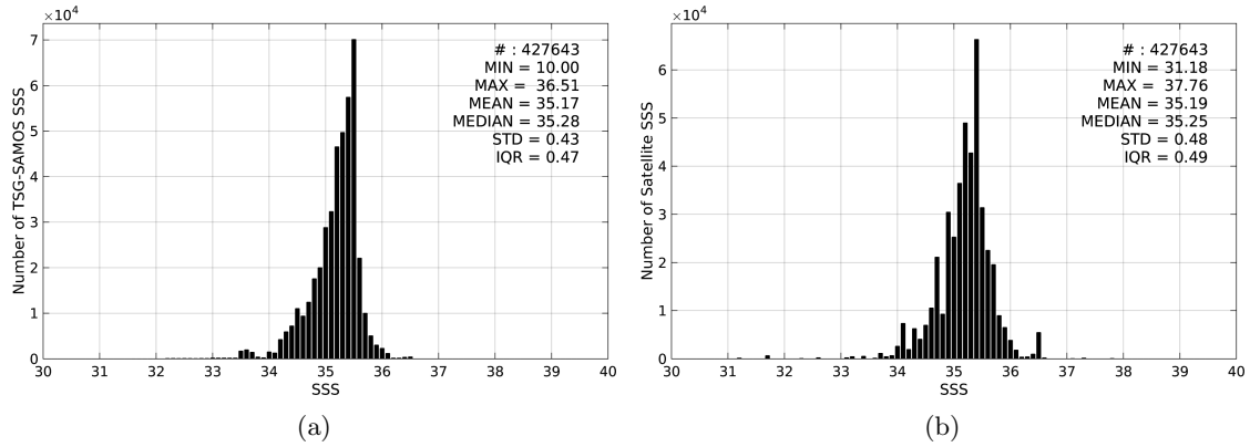
Figure 2: Histograms of SSS from TSG-SAMOS (a) and SMOS-L4-CATDS-CECOS-IFREMER-V2-WEEKLY-0.5DEG (b) considering all match-up pairs per bins of 0.1 over the South Pacific Ocean Pi-MEP region and for the full satellite product period.
