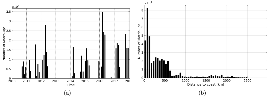
Figure 1: Number of match-ups between TSG-SAMOS and SMOS-L4-CATDS-CECOS-IFREMER-V2-WEEKLY-0.5DEG SSS as a function of time (a) and as function of the distance to coast (b) over the South Pacific Ocean Pi-MEP region and for the full satellite product period.
