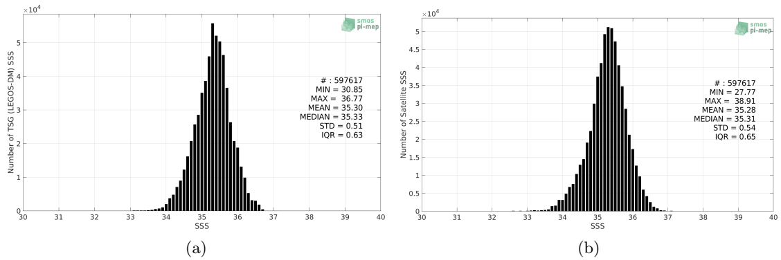
Figure 2: Histograms of SSS from TSG (LEGOS-DM) (a) and SMOS L4 v2 Weekly (CATDS-CECOS-IFREMER) (b) considering all match-up pairs per bins of 0.1 over the South Pacific Ocean Pi-MEP region and for the full satellite product period.
