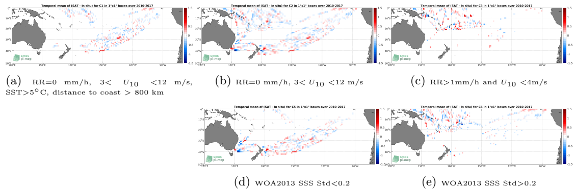
Figure 12: Temporal mean gridded over spatial boxes of size 1^\circ \times 1^\circ of \Delta SSS (SMOS L4 v2 Weekly (CATDS-CECOS-IFREMER) - TSG (LEGOS-DM)) for 5 different subdatasets corresponding to:RR=0 mm/h, 3 < U_{10} < 12 m/s, SST >5^\circ\text{C} , distance to coast > 800 km (a), RR=0 mm/h, 3 < U_{10} < 12 m/s (b), RR >1 mm/h and U_{10} < 4 m/s (c), WOA2013 SSS Std <0.2 (d), WOA2013 SSS Std >0.2 (e).
