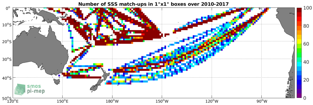
Figure 4: Number of SSS match-ups between TSG (LEGOS-DM) SSS and the SMOS L4 v2 Weekly (CATDS-CECOS-IFREMER) SSS product for the South Pacific Ocean Pi-MEP region over 1^\circ \times 1^\circ boxes and for the full satellite product period.
