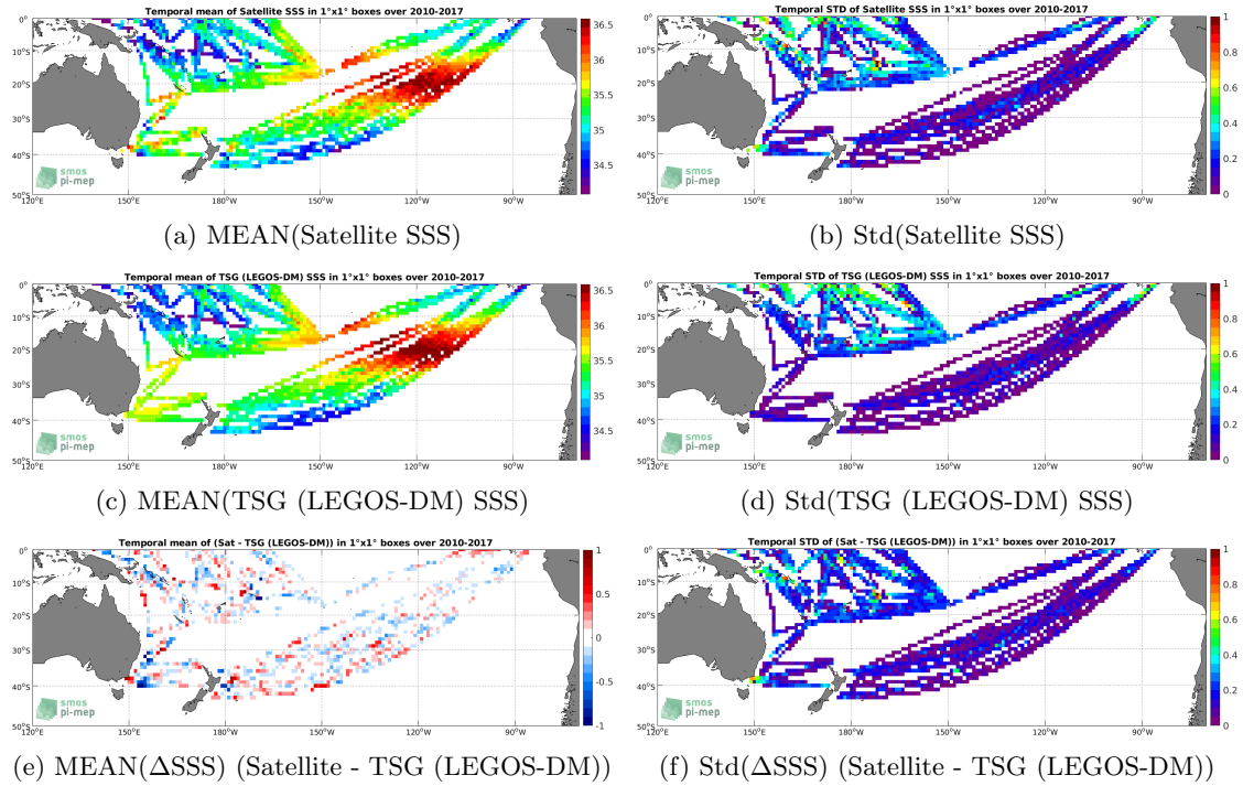
Figure 6: Temporal mean (left) and Std (right) of SSS from SMOS L4 v2 Weekly (CATDS-CECOS-IFREMER) (top), TSG (LEGOS-DM) (middle), and of \Delta SSS (Satellite - TSG (LEGOS-DM)). Only match-up pairs are used to generate these maps.
