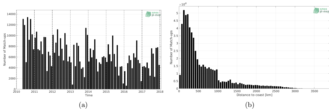
Figure 1: Number of match-ups between TSG (LEGOS-DM) and SMOS L4 v2 Weekly (CATDS-CECOS-IFREMER) SSS as a function of time (a) and as function of the distance to coast (b) over the South Pacific Ocean Pi-MEP region and for the full satellite product period.
