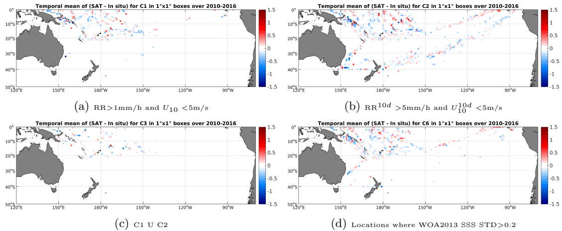
Figure 12: Temporal mean gridded over spatial boxes of size 1^\circ \times 1^\circ of \Delta SSS (SMOS-L4-CATDS-CECOS-IFREMER-V2-WEEKLY-0.5DEG - TSG-LEGOS-DM) for 4 different subdatasets corresponding to: RR > 1\text{mm/h} and U_{10} < 5\text{m/s} (a), RR^{10d} > 5\text{mm/h} and U_{10}^{10d} < 5\text{m/s} (b), C1 U C2 (c), Locations where WOA2013 SSS STD > 0.2 (d).
