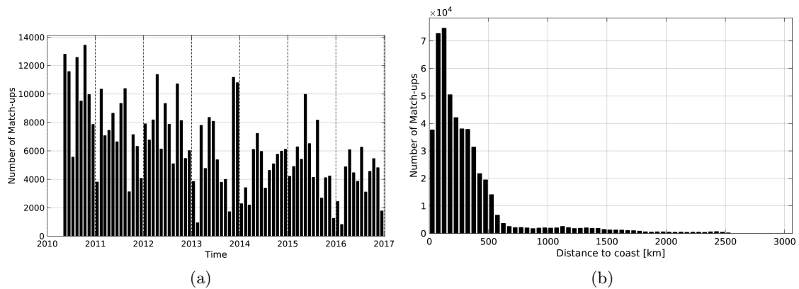
Figure 1: Number of match-ups between TSG-LEGOS-DM and SMOS-L4-CATDS-CECOS-IFREMER-V2-WEEKLY-0.5DEG SSS as a function of time (a) and as function of the distance to coast (b) over the South Pacific Ocean Pi-MEP region and for the full satellite product period.
