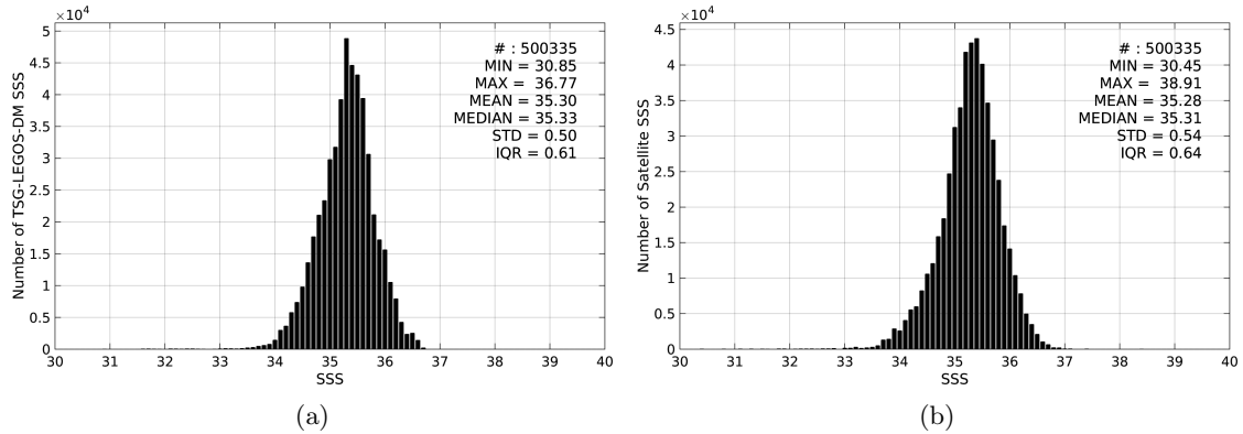
Figure 2: Histograms of SSS from TSG-LEGOS-DM (a) and SMOS-L4-CATDS-CECOS-IFREMER-V2-WEEKLY-0.5DEG (b) considering all match-up pairs per bins of 0.1 over the South Pacific Ocean Pi-MEP region and for the full satellite product period.
