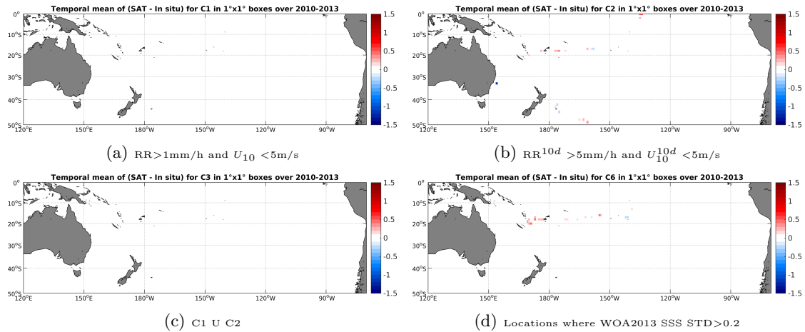
Figure 12: Temporal mean gridded over spatial boxes of size 1^\circ \times 1^\circ of \Delta SSS (SMOS-L4-CATDS-CECOS-IFREMER-V2-WEEKLY-0.5DEG - TSG-GOSUD-Sailing-ship) for 4 different subdatasets corresponding to: RR > 1\text{mm/h} and U_{10} < 5\text{m/s} (a), RR^{10d} > 5\text{mm/h} and U_{10}^{10d} < 5\text{m/s} (b), C1 U C2 (c), Locations where WOA2013 SSS STD > 0.2 (d).
