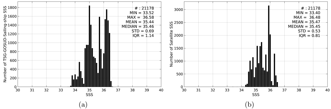
Figure 2: Histograms of SSS from TSG-GOSUD-Sailing-ship (a) and SMOS-L4-CATDS-CECOS-IFREMER-V2-WEEKLY-0.5DEG (b) considering all match-up pairs per bins of 0.1 over the South Pacific Ocean Pi-MEP region and for the full satellite product period.
