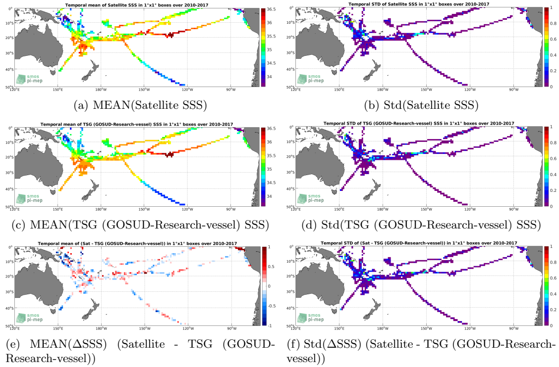
Figure 6: Temporal mean (left) and Std (right) of SSS from SMOS L4 v2 Weekly (CATDS-CECOS-IFREMER) (top), TSG (GOSUD-Research-vessel) (middle), and of \Delta SSS (Satellite - TSG (GOSUD-Research-vessel)). Only match-up pairs are used to generate these maps.
