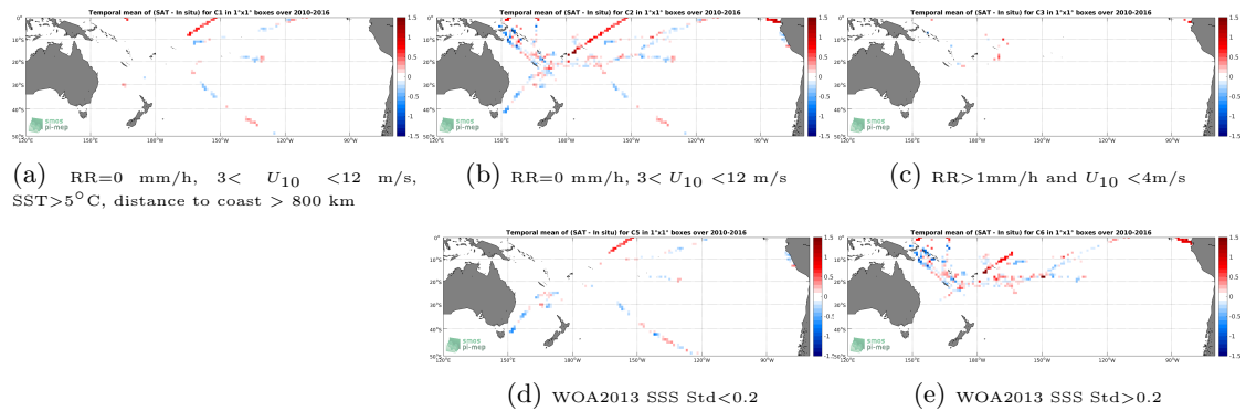
Figure 12: Temporal mean gridded over spatial boxes of size 1^\circ \times 1^\circ of \Delta SSS (SMOS-L4-CATDS-CECOS-IFREMER-V2-WEEKLY-0.5DEG - TSG-GOSUD-Research-vessel) for 5 different sub-datasets corresponding to:RR=0 mm/h, 3 < U_{10} < 12 m/s, SST >5^\circ C , distance to coast > 800 km (a), RR=0 mm/h, 3 < U_{10} < 12 m/s (b), RR >1 mm/h and U_{10} < 4 m/s (c), WOA2013 SSS Std <0.2 (d), WOA2013 SSS Std >0.2 (e).
