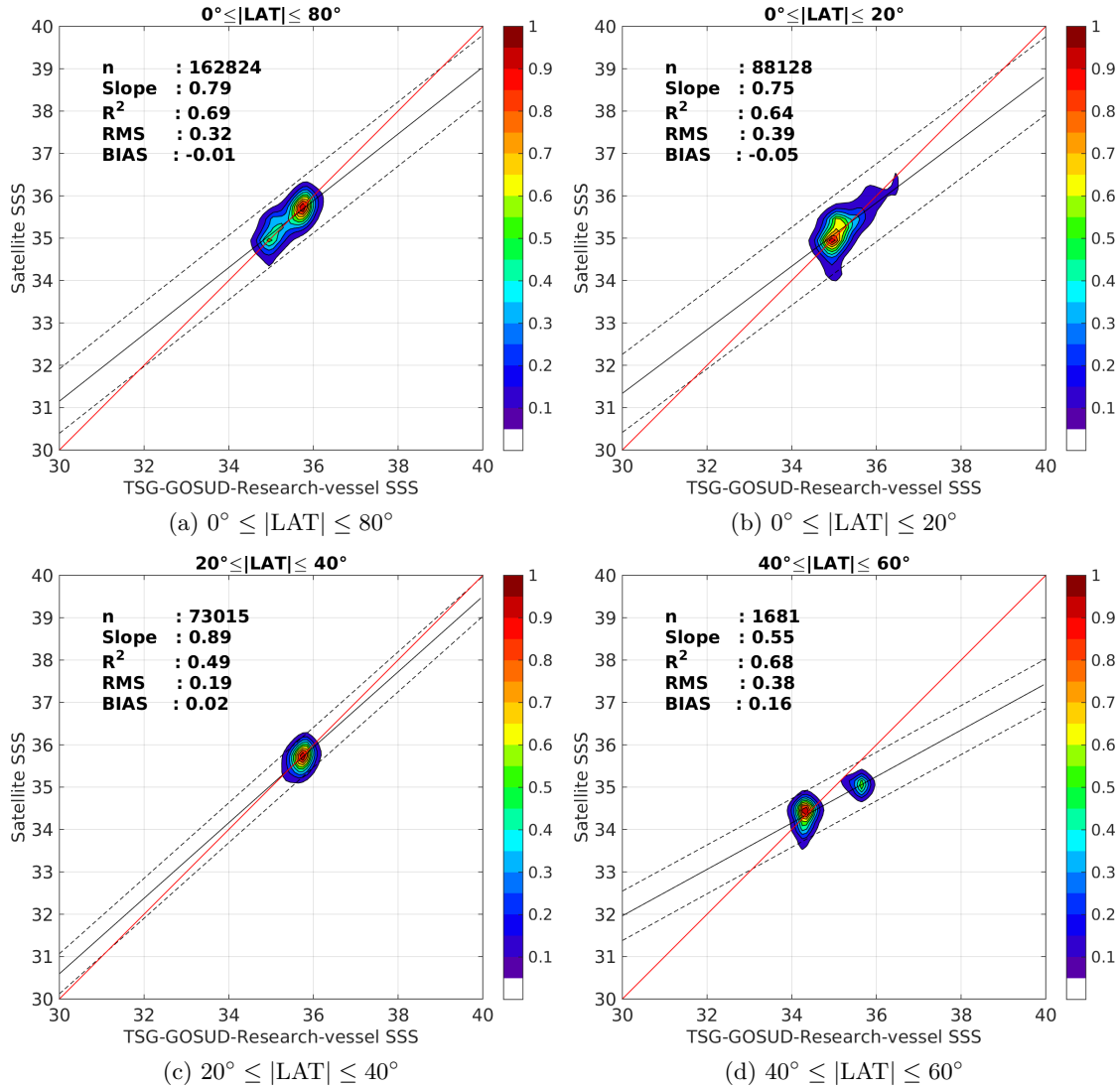
Figure 9: Contour maps of the concentration of SMOS-L4-CATDS-CECOS-IFREMER-V2-WEEKLY-0.5DEG SSS (y-axis) versus TSG-GOSUD-Research-vessel SSS (x-axis) at match-up pairs for different latitude bands. For each plot, the red line shows x=y . The black thin and dashed lines indicate a linear fit through the data cloud and the \pm 95\% confidence levels, respectively. The number match-up pairs n , the slope and R^2 coefficient of the linear fit, the root mean square (RMS) and the mean bias between satellite and in situ data are indicated for each latitude band in each plots.
