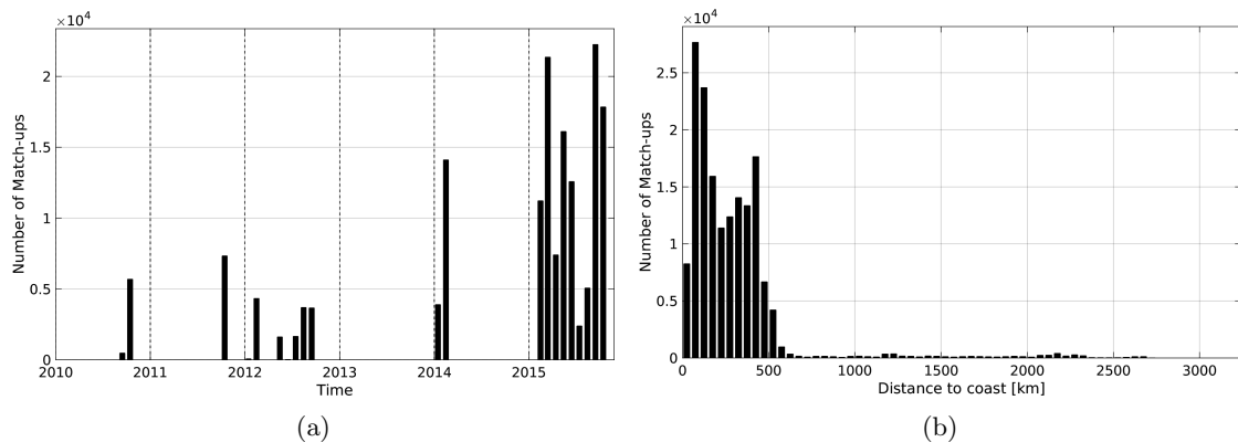
Figure 1: Number of match-ups between TSG-GOSUD-Research-vessel and SMOS-L4-CATDS-CECOS-IFREMER-V2-WEEKLY-0.5DEG SSS as a function of time (a) and as function of the distance to coast (b) over the South Pacific Ocean Pi-MEP region and for the full satellite product period.
