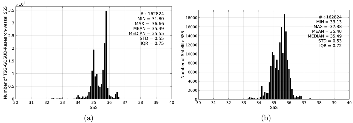
Figure 2: Histograms of SSS from TSG-GOSUD-Research-vessel (a) and SMOS-L4-CATDS-CECOS-IFREMER-V2-WEEKLY-0.5DEG (b) considering all match-up pairs per bins of 0.1 over the South Pacific Ocean Pi-MEP region and for the full satellite product period.
