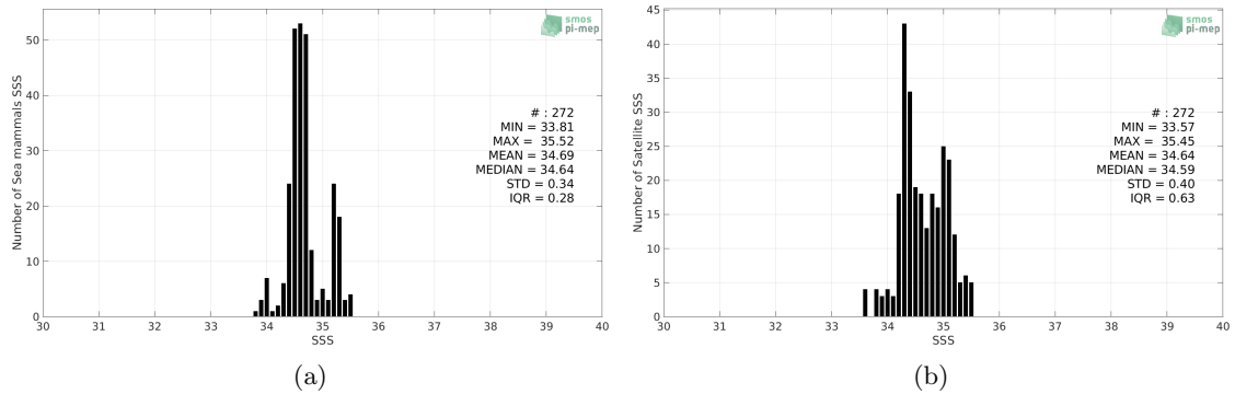
Figure 2: Histograms of SSS from Sea mammals (a) and SMOS L4 v2 Weekly (CATDS-CECOS-IFREMER) (b) considering all match-up pairs per bins of 0.1 over the South Pacific Ocean Pi-MEP region and for the full satellite product period.
