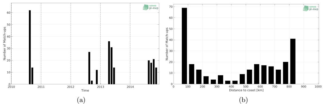
Figure 1: Number of match-ups between Sea mammals and SMOS L4 v2 Weekly (CATDS-CECOS-IFREMER) SSS as a function of time (a) and as function of the distance to coast (b) over the South Pacific Ocean Pi-MEP region and for the full satellite product period.
