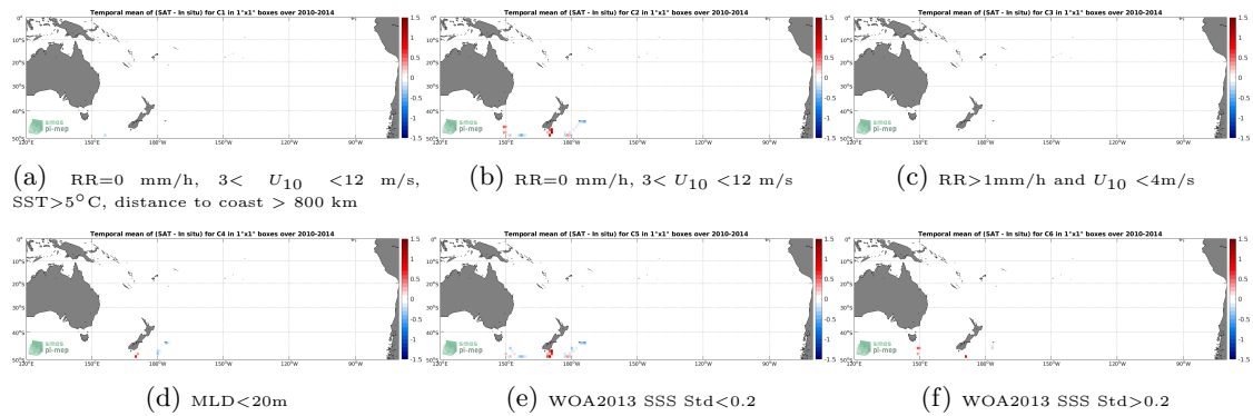
Figure 12: Temporal mean gridded over spatial boxes of size 1^{\circ}\times 1^{\circ} of \Delta\text{SSS} (SMOS L4 v2 Weekly (CATDS-CECOS-IFREMER) - Sea mammals) for 6 different subdatasets corresponding to:RR=0 mm/h, 3 < U_{10} < 12 m/s, SST >5^{\circ}\text{C} , distance to coast > 800 km (a), RR=0 mm/h, 3 < U_{10} < 12 m/s (b), RR >1 mm/h and U_{10} < 4 m/s (c),MLD <20 m (d),WOA2013 SSS Std <0.2 (e),WOA2013 SSS Std >0.2 (f).
