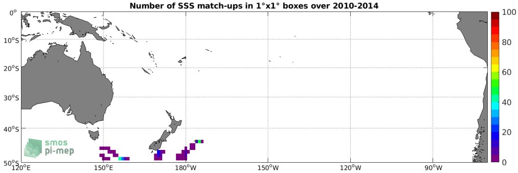
Figure 4: Number of SSS match-ups between Sea mammals SSS and the SMOS L4 v2 Weekly (CATDS-CECOS-IFREMER) SSS product for the South Pacific Ocean Pi-MEP region over 1^\circ \times 1^\circ boxes and for the full satellite product period.
