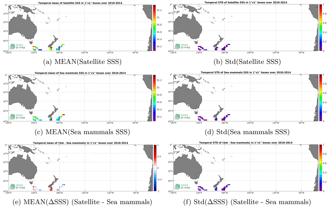
Figure 6: Temporal mean (left) and Std (right) of SSS from SMOS L4 v2 Weekly (CATDS-CECOS-IFREMER) (top), Sea mammals (middle), and of \Delta SSS (Satellite - Sea mammals). Only match-up pairs are used to generate these maps.
