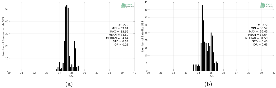
Figure 2: Histograms of SSS from Sea mammals (a) and SMOS-L4-CATDS-CECOS-IFREMER-V2-WEEKLY-0.5DEG (b) considering all match-up pairs per bins of 0.1 over the South Pacific Ocean Pi-MEP region and for the full satellite product period.
