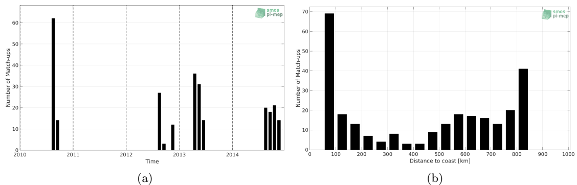
Figure 1: Number of match-ups between Sea mammals and SMOS-L4-CATDS-CECOS-IFREMER-V2-WEEKLY-0.5DEG SSS as a function of time (a) and as function of the distance to coast (b) over the South Pacific Ocean Pi-MEP region and for the full satellite product period.
