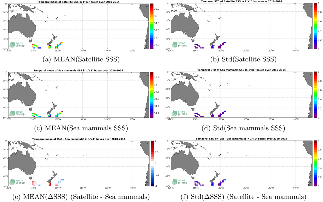
Figure 6: Temporal mean (left) and Std (right) of SSS from SMOS-L4-CATDS-CECOS-IFREMER-V2-WEEKLY-0.5DEG (top), Sea mammals (middle), and of \Delta SSS (Satellite - Sea mammals). Only match-up pairs are used to generate these maps.
