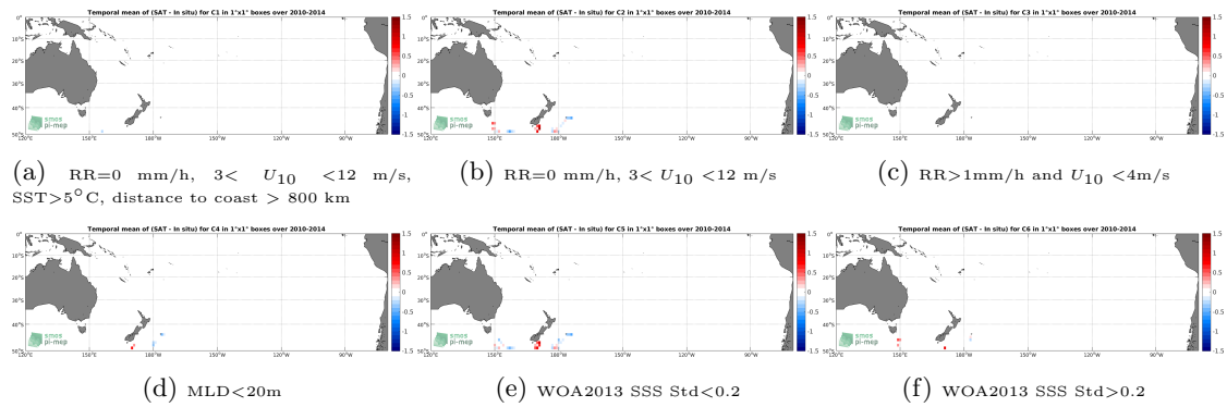
Figure 12: Temporal mean gridded over spatial boxes of size 1^{\circ}\times 1^{\circ} of \Delta\text{SSS} (SMOS-L4-CATDS-CECOS-IFREMER-V2-WEEKLY-0.5DEG - Sea mammals) for 6 different subdatasets corresponding to: \text{RR}=0 mm/h, 3 < U_{10} < 12 m/s, \text{SST} > 5^{\circ}\text{C} , distance to coast > 800 km (a), \text{RR}=0 mm/h, 3 < U_{10} < 12 m/s (b), \text{RR} > 1\text{mm/h} and U_{10} < 4\text{m/s} (c), \text{MLD} < 20\text{m} (d), WOA2013 SSS Std < 0.2 (e), WOA2013 SSS Std > 0.2 (f).
