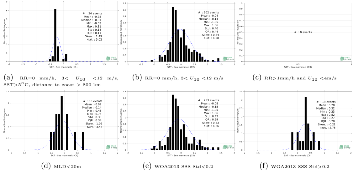
Figure 13: Normalized histogram of \Delta SSS (SMOS-L4-CATDS-CECOS-IFREMER-V2-WEEKLY-0.5DEG - Sea mammals) for 6 different subdatasets corresponding to: RR=0 mm/h, 3 < U_{10} < 12 m/s, SST>5°C, distance to coast > 800 km (a), RR=0 mm/h, 3 < U_{10} < 12 m/s (b), RR>1mm/h and U_{10} < 4 m/s (c), MLD<20m (d), WOA2013 SSS Std<0.2 (e), WOA2013 SSS Std>0.2 (f).
