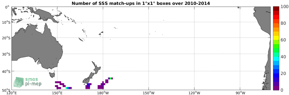
Figure 4: Number of SSS match-ups between Sea mammals SSS and the SMOS-L4-CATDS-CECOS-IFREMER-V2-WEEKLY-0.5DEG SSS product for the South Pacific Ocean Pi-MEP region over 1^\circ \times 1^\circ boxes and for the full satellite product period.
