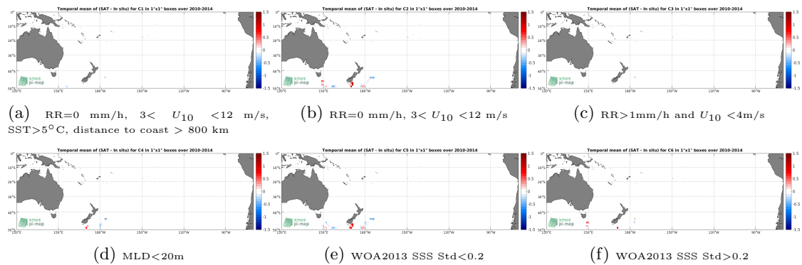
Figure 12: Temporal mean gridded over spatial boxes of size 1^\circ \times 1^\circ of \Delta SSS (SMOS-L4-CATDS-CECOS-IFREMER-V2-WEEKLY-0.5DEG - Sea mammals) for 6 different subdatasets corresponding to: RR=0 mm/h, 3 < U_{10} < 12 m/s, SST > 5^\circ C , distance to coast > 800 km (a), RR=0 mm/h, 3 < U_{10} < 12 m/s (b), RR > 1 mm/h and U_{10} < 4 m/s (c), MLD < 20 m (d), WOA2013 SSS Std < 0.2 (e), WOA2013 SSS Std > 0.2 (f).
