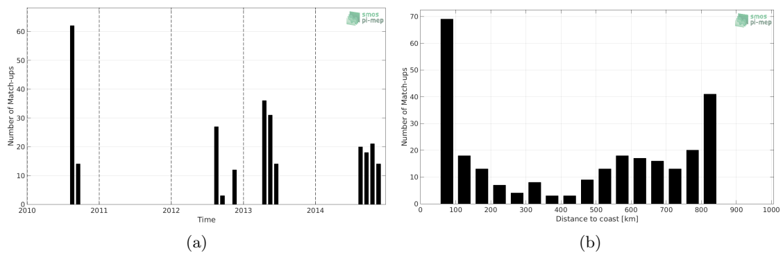
Figure 1: Number of match-ups between Sea mammals and SMOS-4-CATDS-CECOS-IFREMER-V2-WEEKLY-0.5DEG SSS as a function of time (a) and as function of the distance to coast (b) over the South Pacific Ocean Pi-MEP region and for the full satellite product period.
