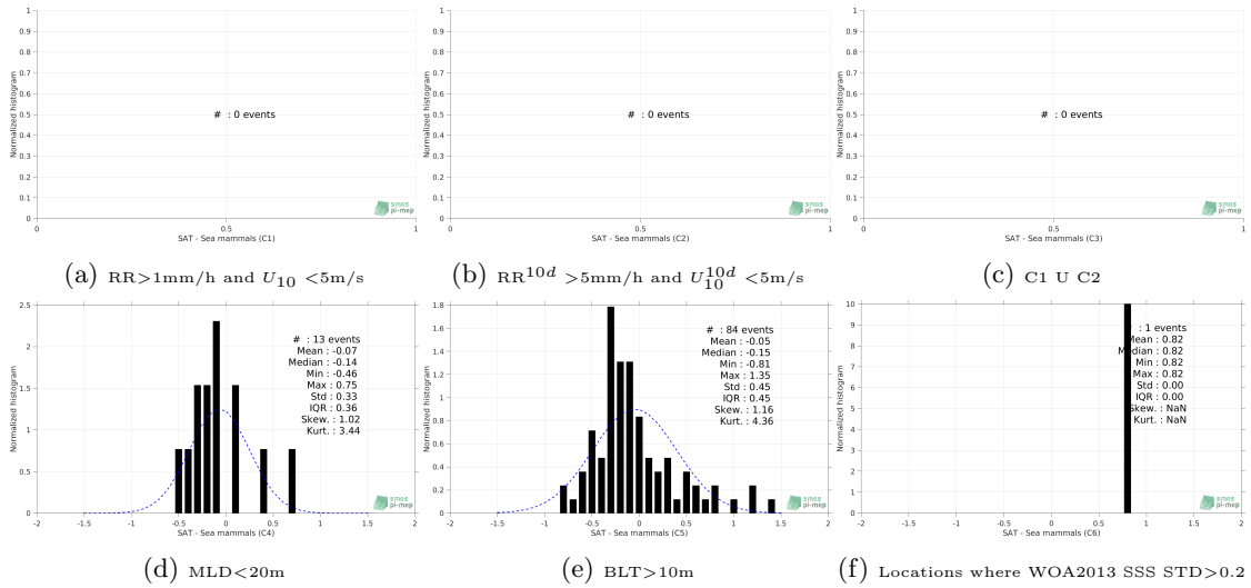
Figure 13: Normalized histogram of \Delta SSS (SMOS-L4-CATDS-CECOS-IFREMER-V2-WEEKLY-0.5DEG - Sea mammals) for 6 different subdatasets corresponding to: RR>1mm/h and U_{10} <5m/s (a), RR^{10d} >5mm/h and U_{10}^{10d} <5m/s (b), C1 U C2 (c),MLD<20m (d),BLT>10m (e),Locations where WOA2013 SSS STD>0.2 (f).
