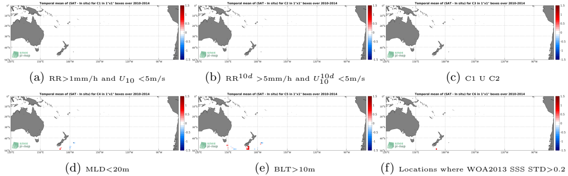
Figure 12: Temporal mean gridded over spatial boxes of size 1°x1° of \Delta SSS (SMOS-L4-CATDS-CECOS-IFREMER-V2-WEEKLY-0.5DEG - Sea mammals) for 6 different subdatasets corresponding to:RR>1mm/h and U_{10} <5m/s (a), RR^{10d} >5mm/h and U_{10}^{10d} <5m/s (b), C1 U C2 (c),MLD<20m (d),BLT>10m (e),Locations where WOA2013 SSS STD>0.2 (f).
