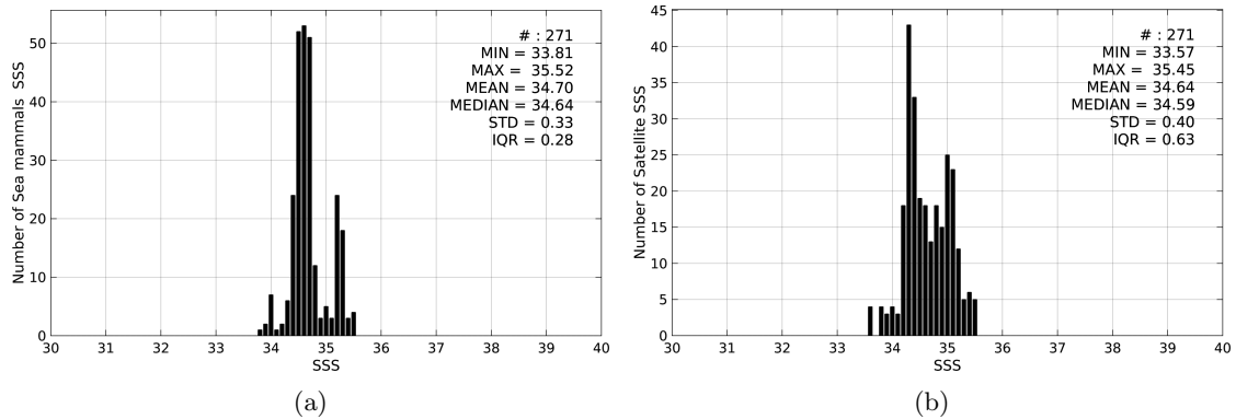
Figure 2: Histograms of SSS from Sea mammals (a) and SMOS-L4-CATDS-CECOS-IFREMER-V2-WEEKLY-0.5DEG (b) considering all match-up pairs per bins of 0.1 over the South Pacific Ocean Pi-MEP region and for the full satellite product period.
