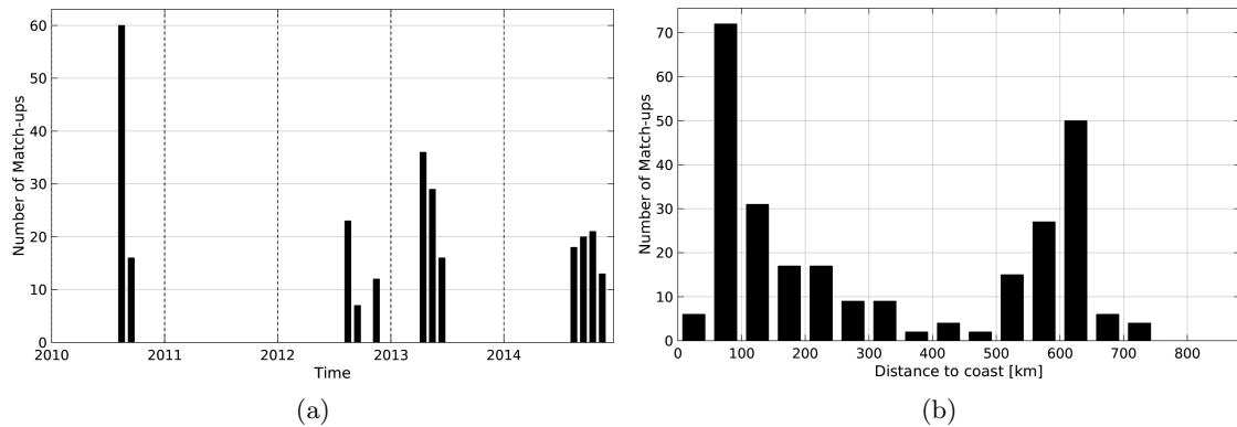
Figure 1: Number of match-ups between Sea mammals and SMOS-L4-CATDS-CECOS-IFREMER-V2-WEEKLY-0.5DEG SSS as a function of time (a) and as function of the distance to coast (b) over the South Pacific Ocean Pi-MEP region and for the full satellite product period.
