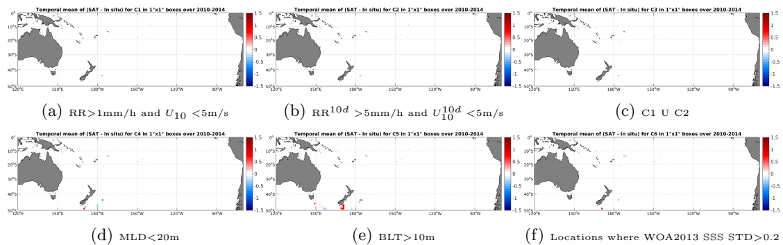
Figure 12: Temporal mean gridded over spatial boxes of size 1^\circ \times 1^\circ of \Delta SSS (SMOS-L4-CATDS-CECOS-IFREMER-V2-WEEKLY-0.5DEG - Sea mammals) for 6 different subdatasets corresponding to:RR >1 mm/h and U_{10} < 5 m/s (a), RR ^{10d} > 5 mm/h and U_{10}^{10d} < 5 m/s (b), C1 U C2 (c),MLD <20 m (d),BLT >10 m (e),Locations where WOA2013 SSS STD >0.2 (f).
