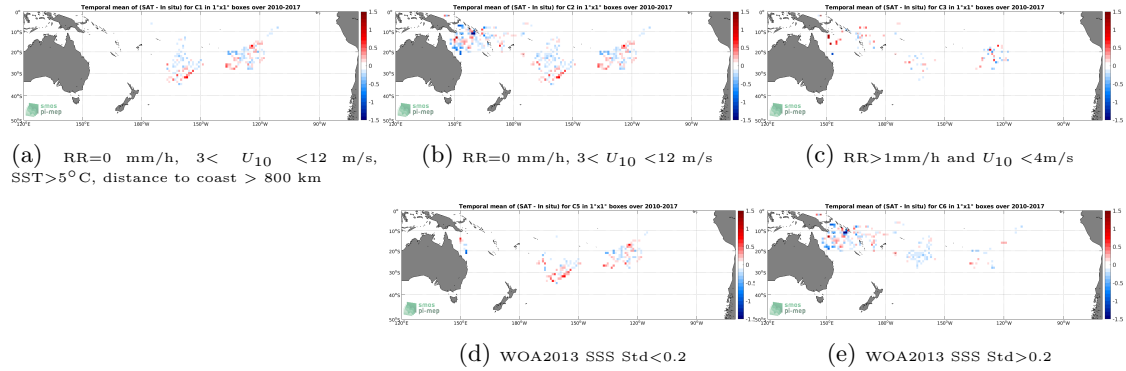
Figure 11: Temporal mean gridded over spatial boxes of size 1^{\circ}\times 1^{\circ} of \Delta\text{SSS} (SMOS L4 v2 Weekly (CATDS-CECOS-IFREMER) - Surface drifters) for 5 different subdatasets corresponding to:RR=0 mm/h, 3 < U_{10} < 12 m/s, SST >5^{\circ}\text{C} , distance to coast > 800 km (a), RR=0 mm/h, 3 < U_{10} < 12 m/s (b), RR >1 mm/h and U_{10} < 4 m/s (c), WOA2013 SSS Std <0.2 (d), WOA2013 SSS Std >0.2 (e).
