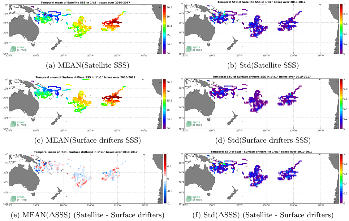
Figure 5: Temporal mean (left) and Std (right) of SSS from SMOS L4 v2 Weekly (CATDS-CECOS-IFREMER) (top), Surface drifters (middle), and of \Delta SSS (Satellite - Surface drifters). Only match-up pairs are used to generate these maps.
