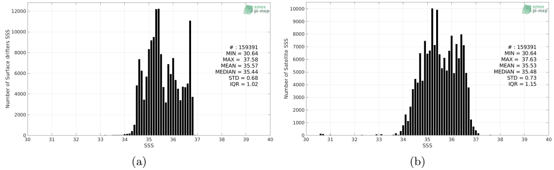
Figure 2: Histograms of SSS from Surface drifters (a) and SMOS L4 v2 Weekly (CATDS-CECOS-IFREMER) (b) considering all match-up pairs per bins of 0.1 over the South Pacific Ocean Pi-MEP region and for the full satellite product period.
