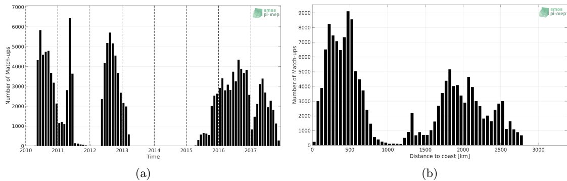
Figure 1: Number of match-ups between Surface drifters and SMOS L4 v2 Weekly (CATDS-CECOS-IFREMER) SSS as a function of time (a) and as function of the distance to coast (b) over the South Pacific Ocean Pi-MEP region and for the full satellite product period.
