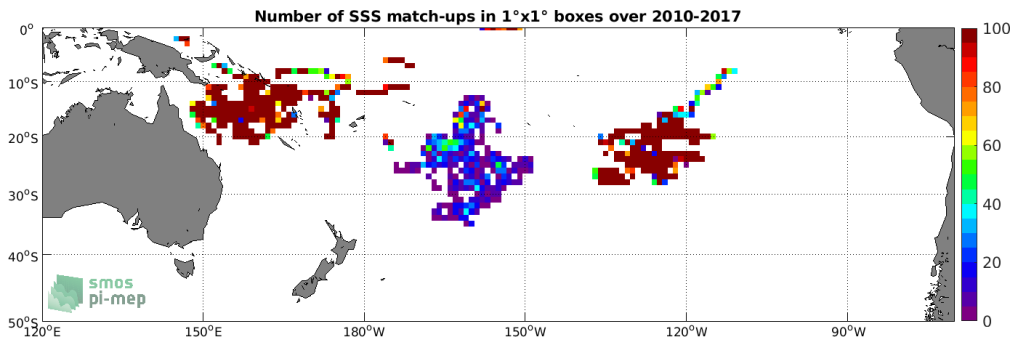
Figure 3: Number of SSS match-ups between Surface drifters SSS and the SMOS L4 v2 Weekly (CATDS-CECOS-IFREMER) SSS product for the South Pacific Ocean Pi-MEP region over 1^\circ \times 1^\circ boxes and for the full satellite product period.
