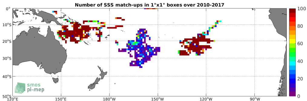
Figure 3: Number of SSS match-ups between Surface drifters SSS and the SMOS L4 v2 Weekly (CATDS-CECOS-IFREMER) SSS product for the South Pacific Ocean Pi-MEP region over 1°x1° boxes and for the full satellite product period.
