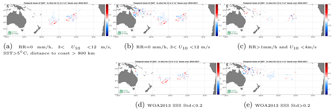
Figure 11: Temporal mean gridded over spatial boxes of size 1^{\circ}\times 1^{\circ} of \Delta\text{SSS} (SMOS-L4-CATDS-CECOS-IFREMER-V2-WEEKLY-0.5DEG - Surface drifters) for 5 different subdatasets corresponding to:RR=0 mm/h, 3 < U_{10} < 12 m/s, SST >5^{\circ}\text{C} , distance to coast > 800 km (a), RR=0 mm/h, 3 < U_{10} < 12 m/s (b), RR >1 mm/h and U_{10} < 4 m/s (c), WOA2013 SSS Std <0.2 (d), WOA2013 SSS Std >0.2 (e).
