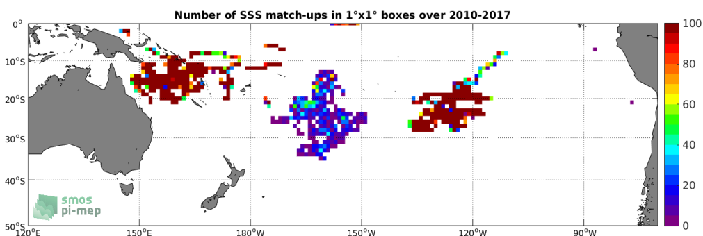
Figure 3: Number of SSS match-ups between Surface drifters SSS and the SMOS-L4-CATDS-CECOS-IFREMER-V2-WEEKLY-0.5DEG SSS product for the South Pacific Ocean Pi-MEP region over 1°x1° boxes and for the full satellite product period.
