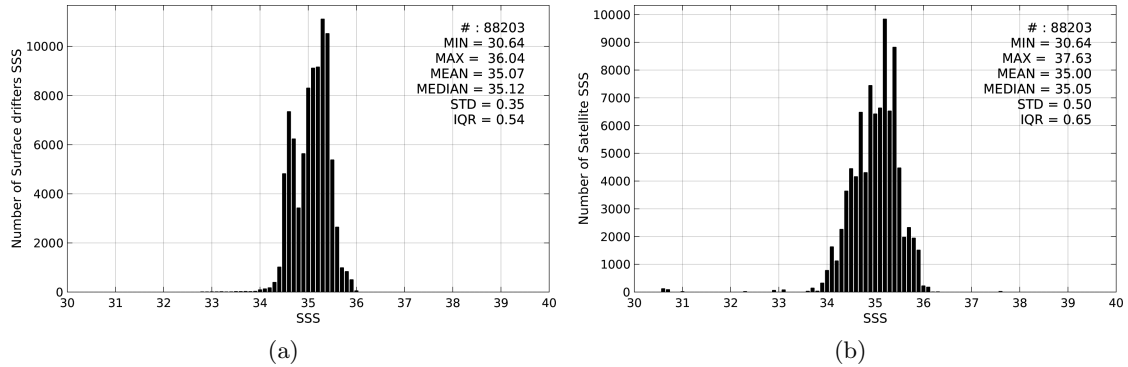
Figure 2: Histograms of SSS from Surface drifters (a) and SMOS-L4-CATDS-CECOS-IFREMER-V2-WEEKLY-0.5DEG (b) considering all match-up pairs per bins of 0.1 over the South Pacific Ocean Pi-MEP region and for the full satellite product period.
