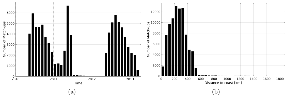
Figure 1: Number of match-ups between Surface drifters and SMOS-L4-CATDS-CECOS-IFREMER-V2-WEEKLY-0.5DEG SSS as a function of time (a) and as function of the distance to coast (b) over the South Pacific Ocean Pi-MEP region and for the full satellite product period.
