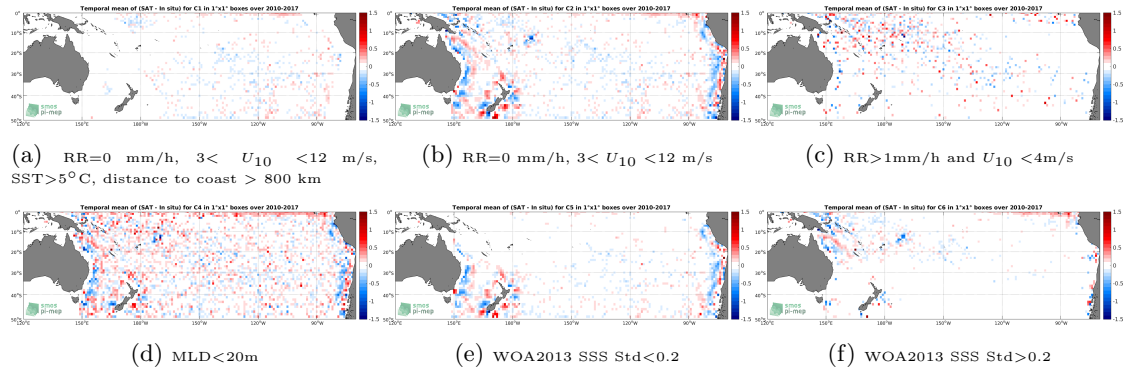
Figure 12: Temporal mean gridded over spatial boxes of size 1^\circ \times 1^\circ of \Delta SSS (SMOS-L4-CATDS-CECOS-IFREMER-V2-WEEKLY-0.5DEG - Argo) for 6 different subdatasets corresponding to: RR=0 mm/h, 3 < U_{10} < 12 m/s, SST > 5^\circ C , distance to coast > 800 km (a), RR=0 mm/h, 3 < U_{10} < 12 m/s (b), RR > 1 mm/h and U_{10} < 4 m/s (c), MLD < 20 m (d), WOA2013 SSS Std < 0.2 (e), WOA2013 SSS Std > 0.2 (f).
