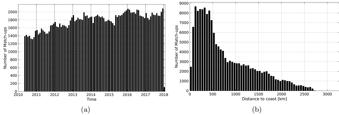
Figure 1: Number of match-ups between Argo and SMOS-L4-CATDS-CECOS-IFREMER-V2-WEEKLY-0.5DEG SSS as a function of time (a) and as function of the distance to coast (b) over the South Pacific Ocean Pi-MEP region and for the full satellite product period.
