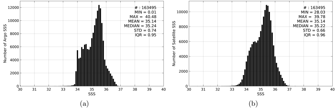
Figure 2: Histograms of SSS from Argo (a) and SMOS-L4-CATDS-CECOS-IFREMER-V2-WEEKLY-0.5DEG (b) considering all match-up pairs per bins of 0.1 over the South Pacific Ocean Pi-MEP region and for the full satellite product period.
