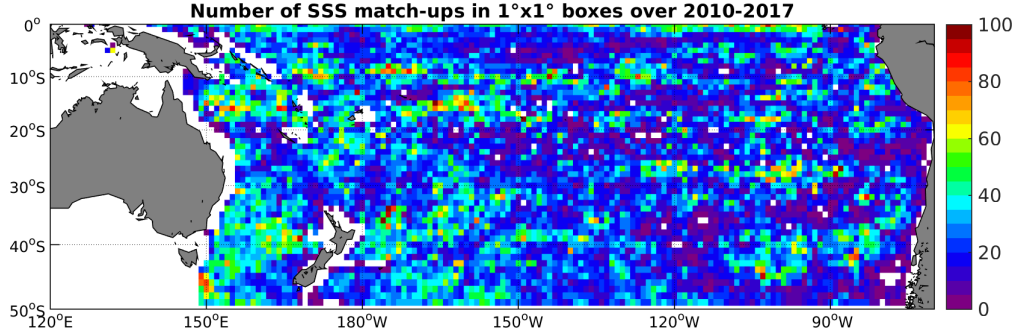
Figure 4: Number of SSS match-ups between Argo SSS and the SMOS-L4-CATDS-CECOS-IFREMER-V2-WEEKLY-0.5DEG SSS product for the South Pacific Ocean Pi-MEP region over 1^\circ \times 1^\circ boxes and for the full satellite product period.
