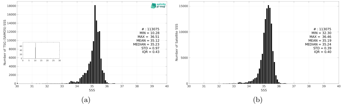
Figure 3: Histograms of SSS from TSG (SAMOS) (a) and SMOS SSS L4 v2 - Daily (BEC) (b) considering all match-up pairs per bins of 0.1 over the South Pacific Ocean Pi-MEP region and for the full satellite product period.
