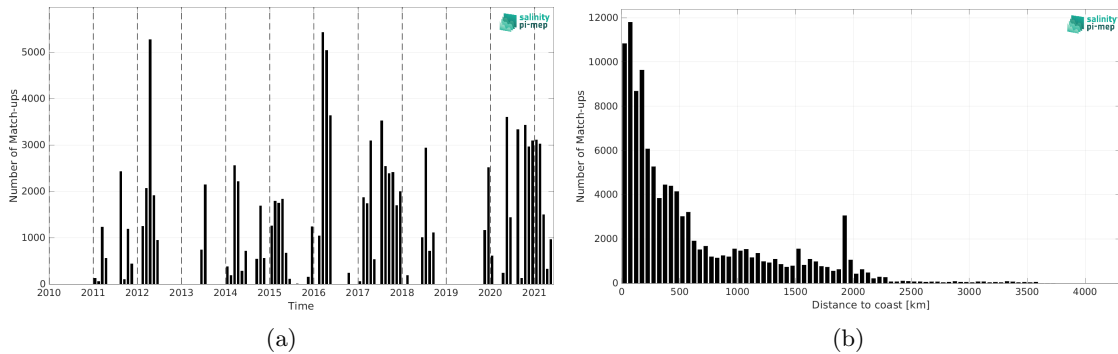
Figure 2: Number of match-ups between TSG (SAMOS) and SMOS SSS L4 v2 - Daily (BEC) SSS as a function of time (a) and as function of the distance to coast (b) over the South Pacific Ocean Pi-MEP region and for the full satellite product period.
