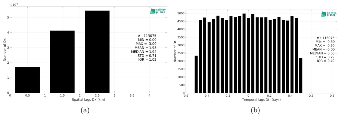
Figure 6: Histograms of the spatial (a) and temporal (b) lags between the location/time of the TSG (SAMOS) measurement and the date of the corresponding SMOS SSS L4 v2 - Daily (BEC) SSS pixel.
