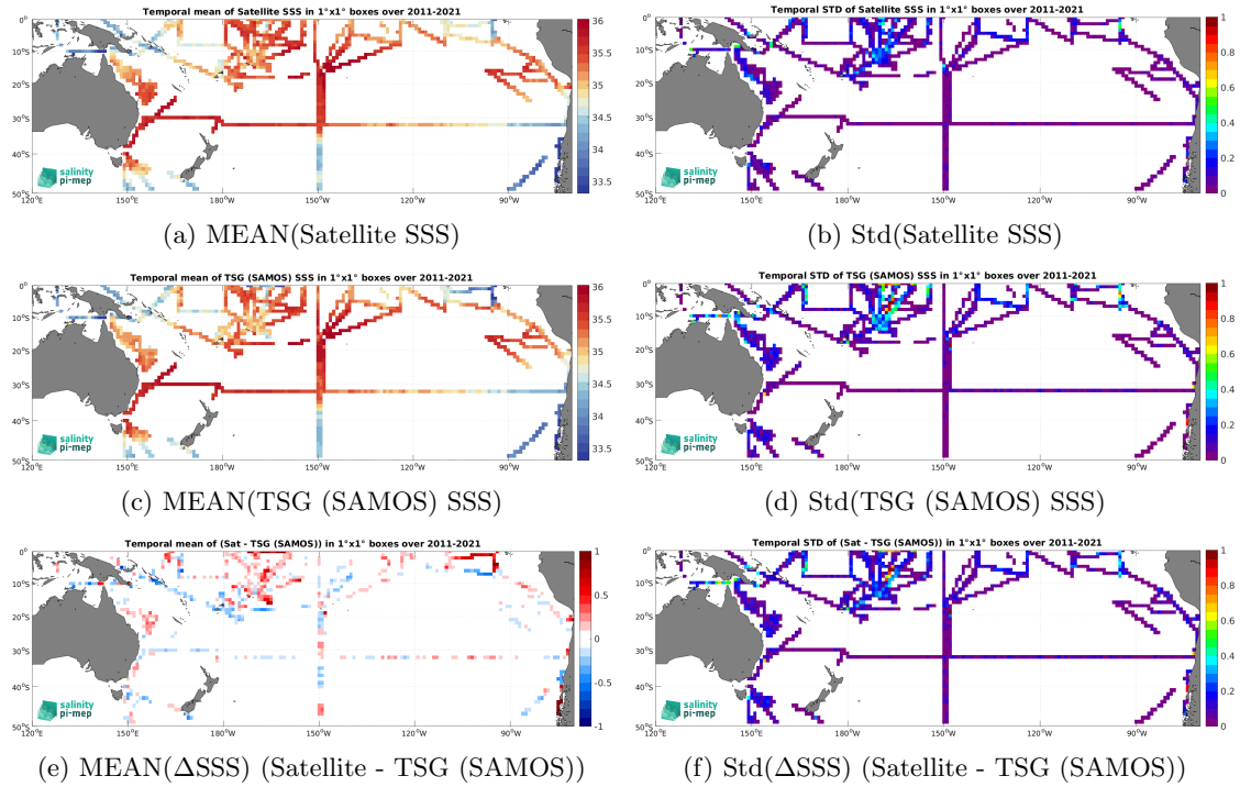
Figure 7: Temporal mean (left) and Std (right) of SSS from SMOS SSS L4 v2 - Daily (BEC) (top), TSG (SAMOS) (middle), and of \Delta SSS (Satellite - TSG (SAMOS)). Only match-up pairs are used to generate these maps.
