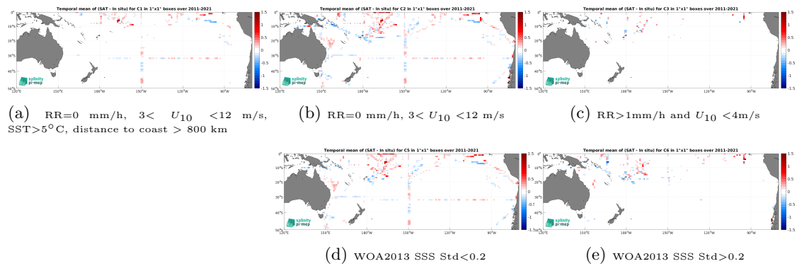
Figure 14: Temporal mean gridded over spatial boxes of size 1^\circ \times 1^\circ of \Delta\text{SSS} (SMOS SSS L4 v2 - Daily (BEC) - TSG (SAMOS)) for 5 different subdatasets corresponding to:RR=0 mm/h, 3 < U_{10} < 12 m/s, SST >5^\circ\text{C} , distance to coast > 800 km (a), RR=0 mm/h, 3 < U_{10} < 12 m/s (b), RR >1 mm/h and U_{10} < 4 m/s (c), WOA2013 SSS Std <0.2 (d), WOA2013 SSS Std >0.2 (e).
