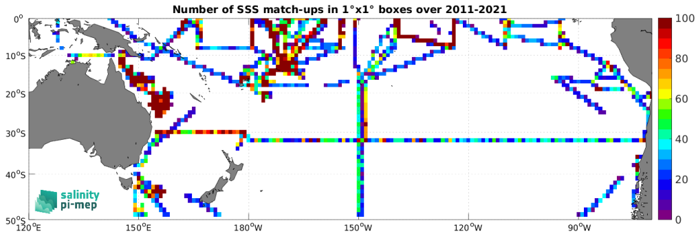
Figure 5: Number of SSS match-ups between TSG (SAMOS) SSS and the SMOS SSS L4 v2 - Daily (BEC) SSS product for the South Pacific Ocean Pi-MEP region over 1^\circ \times 1^\circ boxes and for the full satellite product period.
