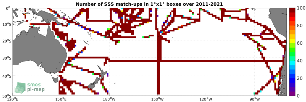
Figure 4: Number of SSS match-ups between TSG (SAMOS) SSS and the SMOS SSS L4 v2 - Daily (BEC) SSS product for the South Pacific Ocean Pi-MEP region over 1^\circ \times 1^\circ boxes and for the full satellite product period.
