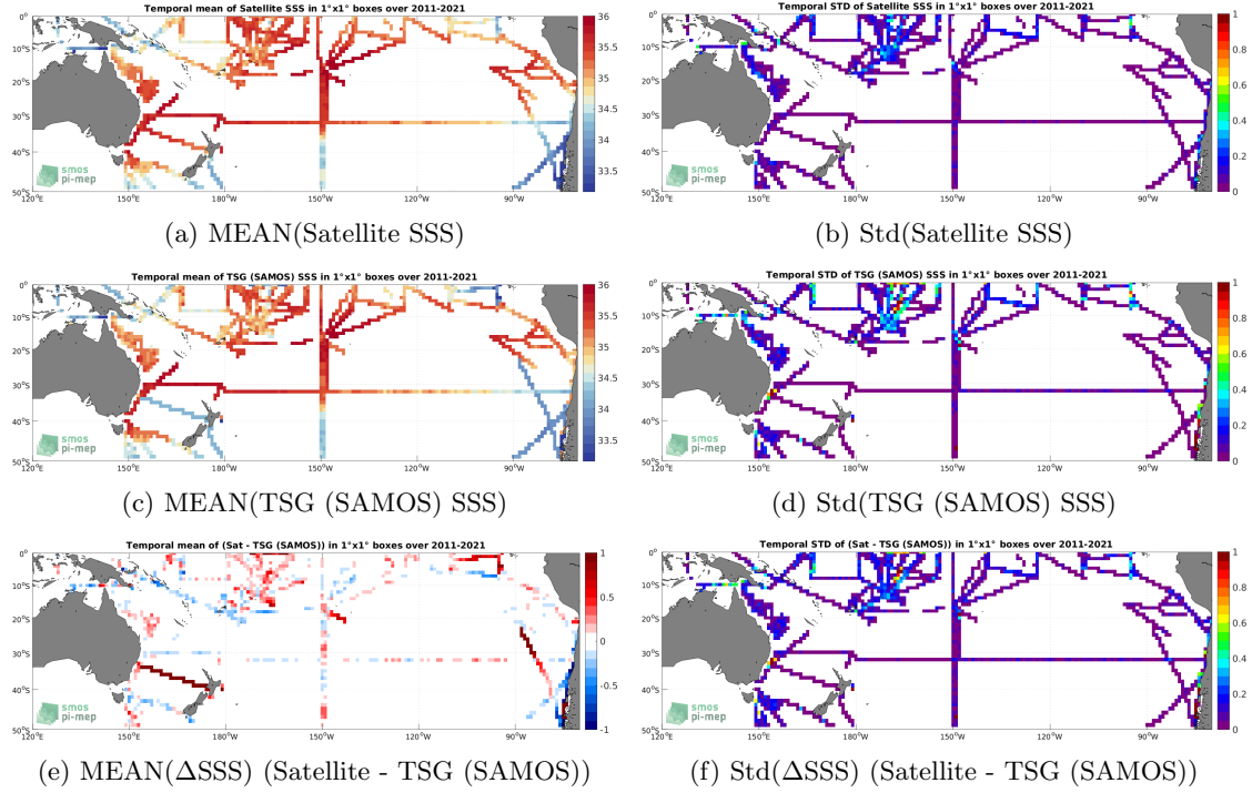
Figure 6: Temporal mean (left) and Std (right) of SSS from SMOS SSS L4 v2 - Daily (BEC) (top), TSG (SAMOS) (middle), and of \Delta SSS (Satellite - TSG (SAMOS)). Only match-up pairs are used to generate these maps.
