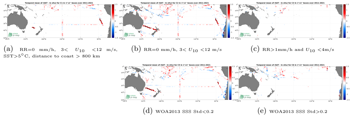
Figure 12: Temporal mean gridded over spatial boxes of size 1^\circ \times 1^\circ of \Delta SSS (SMOS SSS L4 v2 - Daily (BEC) - TSG (SAMOS)) for 5 different subdatasets corresponding to:RR=0 mm/h, 3 < U_{10} < 12 m/s, SST >5^\circ\text{C} , distance to coast > 800 km (a), RR=0 mm/h, 3 < U_{10} < 12 m/s (b), RR >1 mm/h and U_{10} < 4 m/s (c), WOA2013 SSS Std <0.2 (d), WOA2013 SSS Std >0.2 (e).
