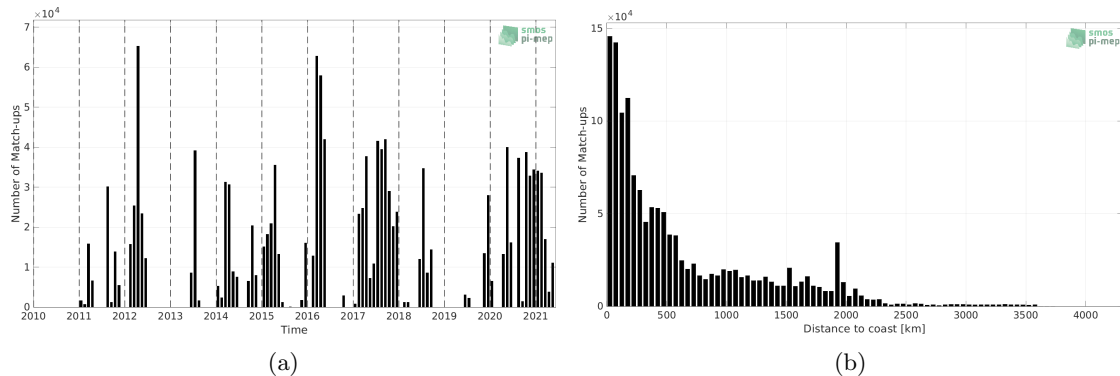
Figure 1: Number of match-ups between TSG (SAMOS) and SMOS SSS L4 v2 - Daily (BEC) SSS as a function of time (a) and as function of the distance to coast (b) over the South Pacific Ocean Pi-MEP region and for the full satellite product period.
