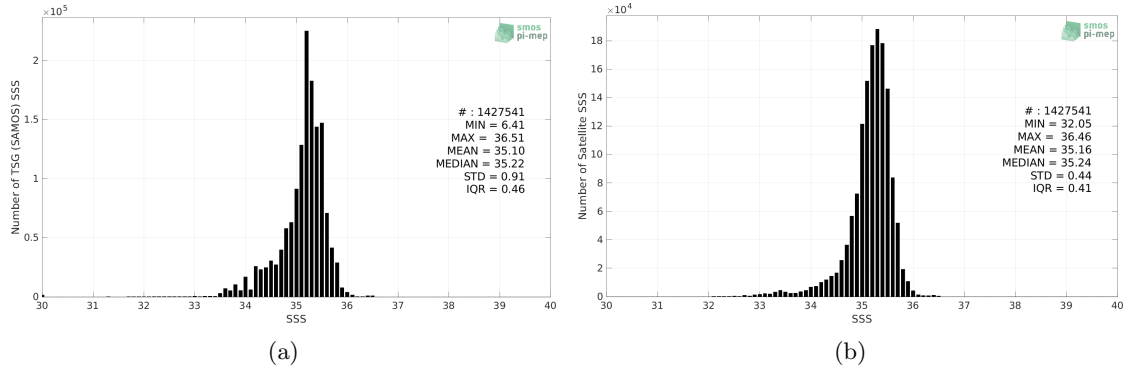
Figure 2: Histograms of SSS from TSG (SAMOS) (a) and SMOS SSS L4 v2 - Daily (BEC) (b) considering all match-up pairs per bins of 0.1 over the South Pacific Ocean Pi-MEP region and for the full satellite product period.
