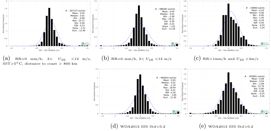
Figure 13: Normalized histogram of \Delta SSS (SMOS SSS L4 v2 - Daily (BEC) - TSG (SAMOS)) for 5 different subdatasets corresponding to: RR=0 mm/h, 3 < U_{10} < 12 m/s, SST > 5°C, distance to coast > 800 km (a), RR=0 mm/h, 3 < U_{10} < 12 m/s (b), RR > 1mm/h and U_{10} < 4 m/s (c), WOA2013 SSS Std < 0.2 (d), WOA2013 SSS Std > 0.2 (e).
