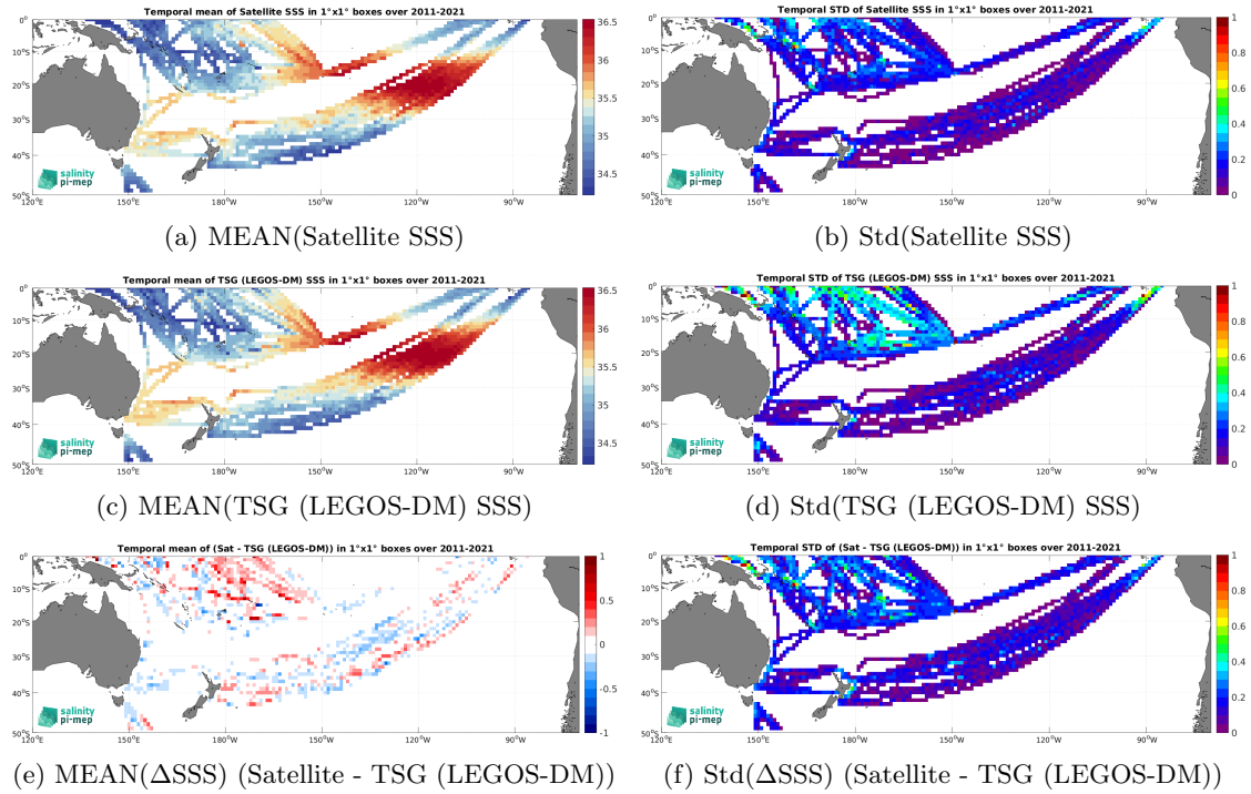
Figure 7: Temporal mean (left) and Std (right) of SSS from SMOS SSS L4 v2 - Daily (BEC) (top), TSG (LEGOS-DM) (middle), and of \Delta SSS (Satellite - TSG (LEGOS-DM)). Only match-up pairs are used to generate these maps.
