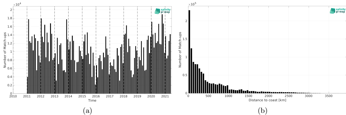
Figure 2: Number of match-ups between TSG (LEGOS-DM) and SMOS SSS L4 v2 - Daily (BEC) SSS as a function of time (a) and as function of the distance to coast (b) over the South Pacific Ocean Pi-MEP region and for the full satellite product period.
