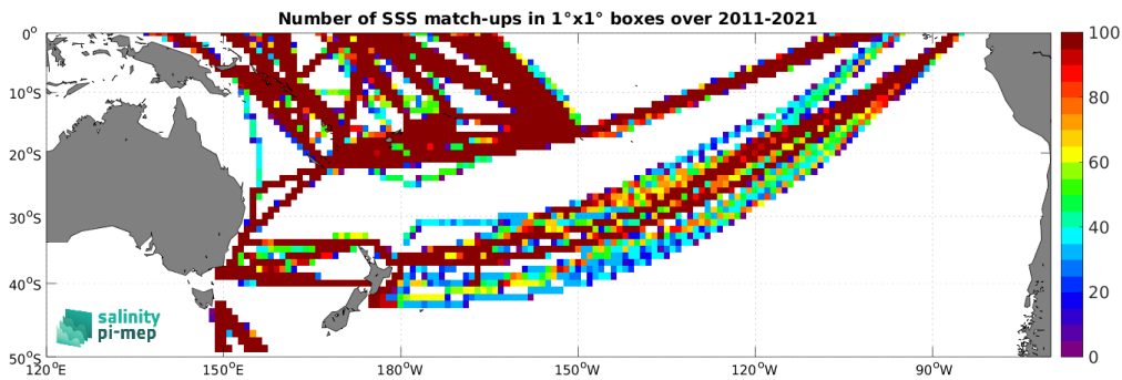
Figure 5: Number of SSS match-ups between TSG (LEGOS-DM) SSS and the SMOS SSS L4 v2 - Daily (BEC) SSS product for the South Pacific Ocean Pi-MEP region over 1^\circ \times 1^\circ boxes and for the full satellite product period.
