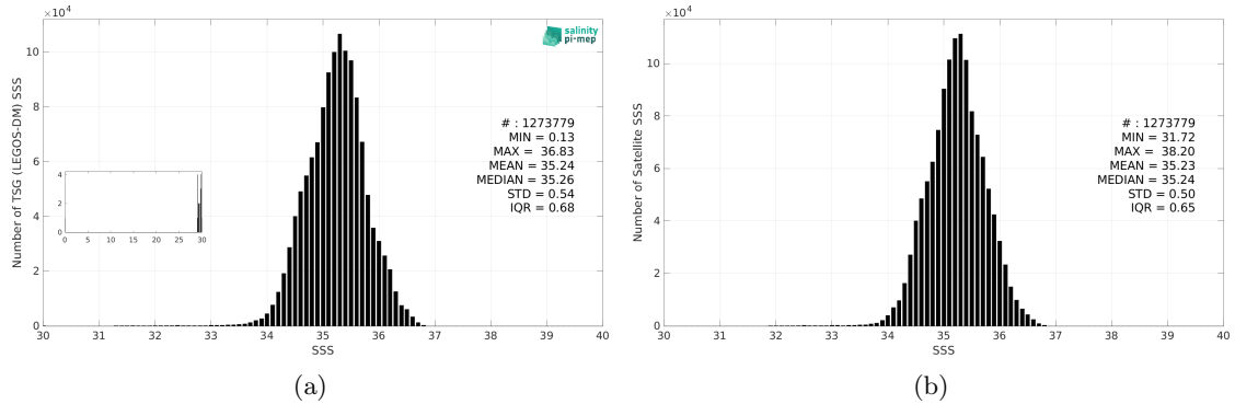
Figure 3: Histograms of SSS from TSG (LEGOS-DM) (a) and SMOS SSS L4 v2 - Daily (BEC) (b) considering all match-up pairs per bins of 0.1 over the South Pacific Ocean Pi-MEP region and for the full satellite product period.
