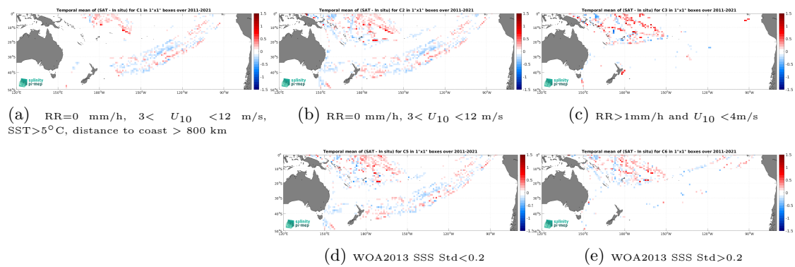
Figure 14: Temporal mean gridded over spatial boxes of size 1^\circ \times 1^\circ of \Delta SSS (SMOS SSS L4 v2 - Daily (BEC) - TSG (LEGOS-DM)) for 5 different subdatasets corresponding to:RR=0 mm/h, 3 < U_{10} < 12 m/s, SST >5^\circ\text{C} , distance to coast > 800 km (a), RR=0 mm/h, 3 < U_{10} < 12 m/s (b), RR >1 mm/h and U_{10} < 4 m/s (c), WOA2013 SSS Std <0.2 (d), WOA2013 SSS Std >0.2 (e).
