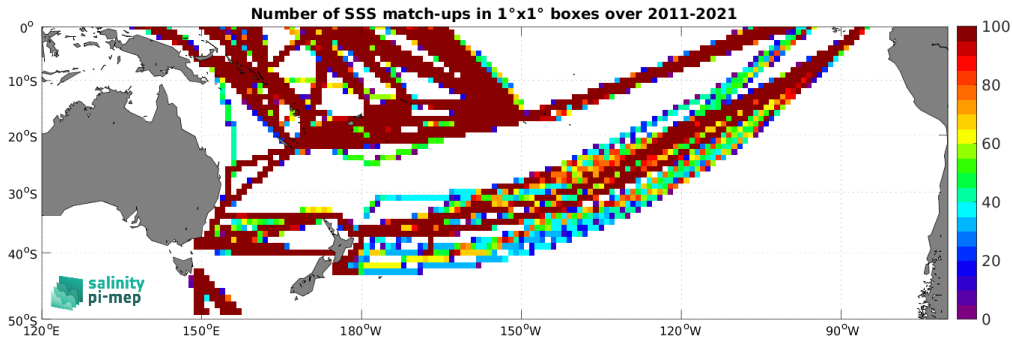
Figure 4: Number of SSS match-ups between TSG (LEGOS-DM) SSS and the SMOS SSS L4 v2 - Daily (BEC) SSS product for the South Pacific Ocean Pi-MEP region over 1^\circ \times 1^\circ boxes and for the full satellite product period.
