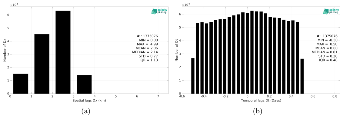
Figure 5: Histograms of the spatial (a) and temporal (b) lags between the location/time of the TSG (LEGOS-DM) measurement and the date of the corresponding SMOS SSS L4 v2 - Daily (BEC) SSS pixel.
