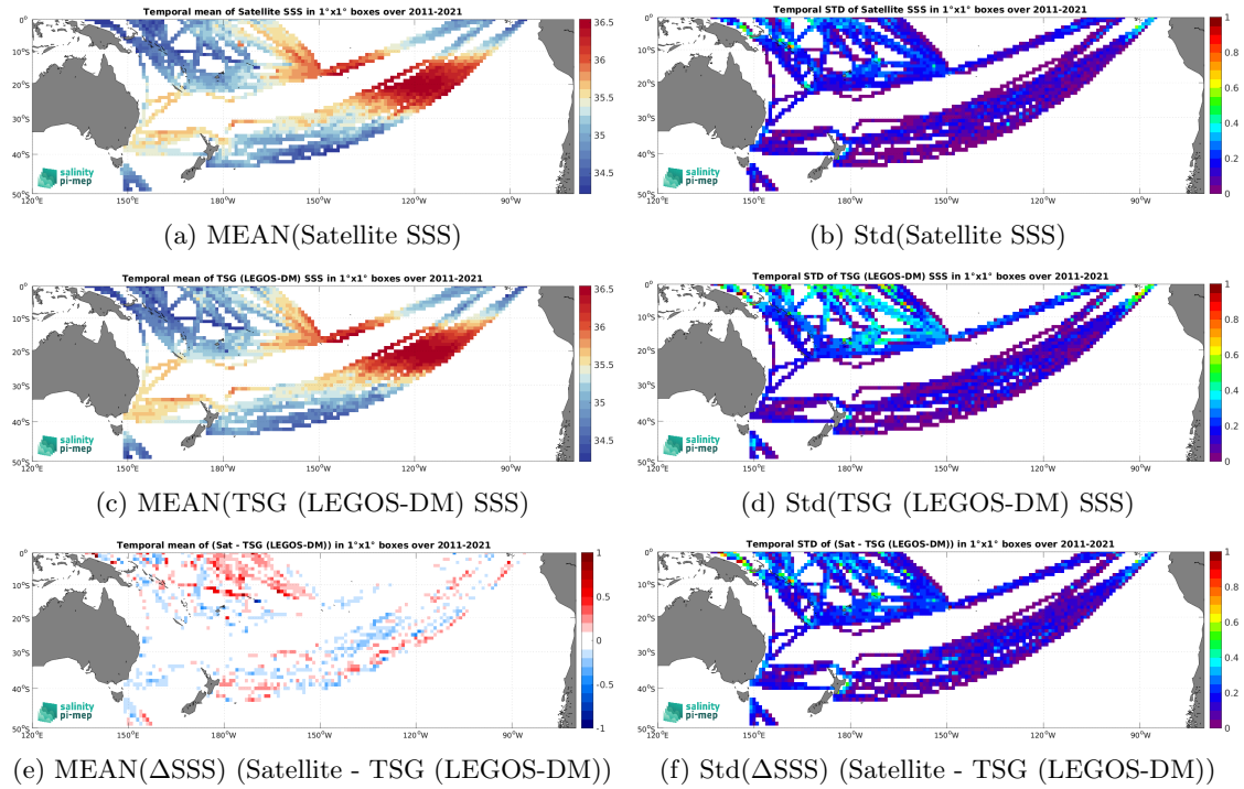
Figure 6: Temporal mean (left) and Std (right) of SSS from SMOS SSS L4 v2 - Daily (BEC) (top), TSG (LEGOS-DM) (middle), and of \Delta SSS (Satellite - TSG (LEGOS-DM)). Only match-up pairs are used to generate these maps.
