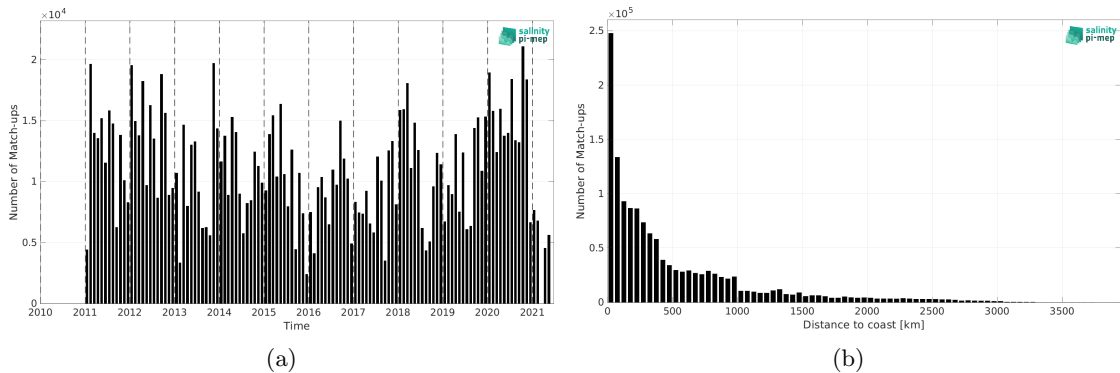
Figure 1: Number of match-ups between TSG (LEGOS-DM) and SMOS SSS L4 v2 - Daily (BEC) SSS as a function of time (a) and as function of the distance to coast (b) over the South Pacific Ocean Pi-MEP region and for the full satellite product period.
