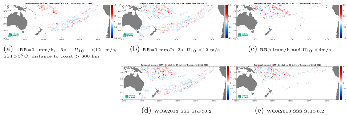
Figure 12: Temporal mean gridded over spatial boxes of size 1^\circ \times 1^\circ of \Delta SSS (SMOS SSS L4 v2 - Daily (BEC) - TSG (LEGOS-DM)) for 5 different subdatasets corresponding to:RR=0 mm/h, 3 < U_{10} < 12 m/s, SST >5^\circ\text{C} , distance to coast > 800 km (a), RR=0 mm/h, 3 < U_{10} < 12 m/s (b), RR >1 mm/h and U_{10} < 4 m/s (c), WOA2013 SSS Std <0.2 (d), WOA2013 SSS Std >0.2 (e).
