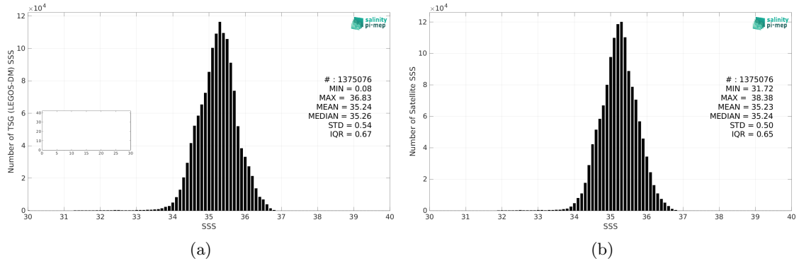
Figure 2: Histograms of SSS from TSG (LEGOS-DM) (a) and SMOS SSS L4 v2 - Daily (BEC) (b) considering all match-up pairs per bins of 0.1 over the South Pacific Ocean Pi-MEP region and for the full satellite product period.
