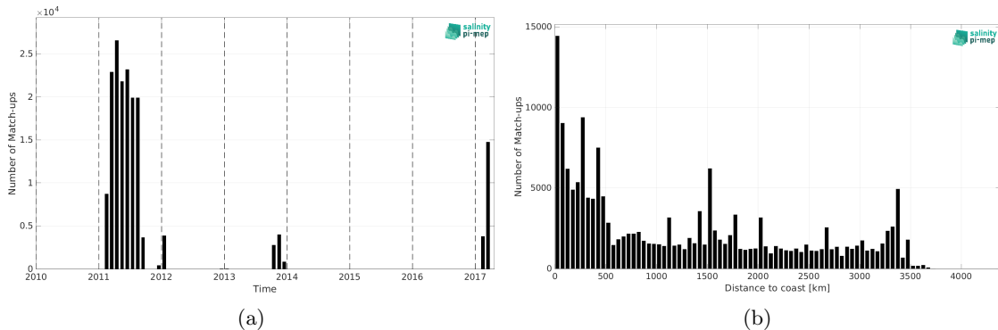
Figure 2: Number of match-ups between TSG (GOSUD-Sailing-ship) and SMOS SSS L4 v2 - Daily (BEC) SSS as a function of time (a) and as function of the distance to coast (b) over the South Pacific Ocean Pi-MEP region and for the full satellite product period.
