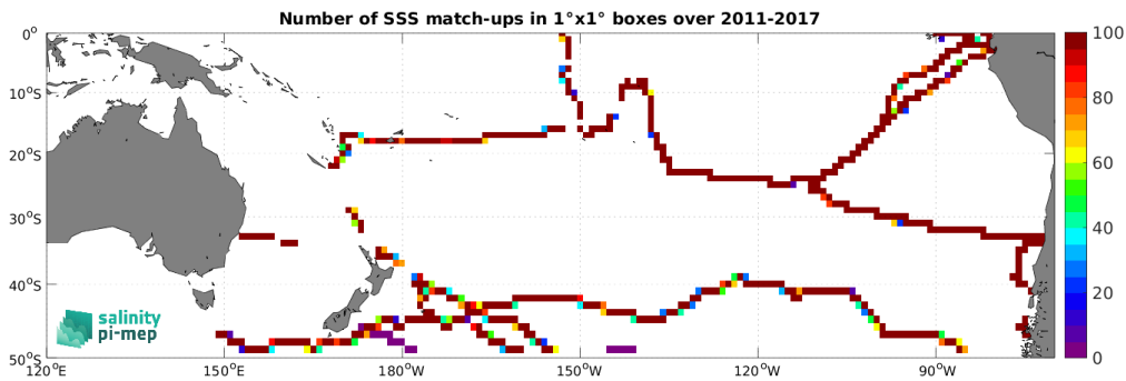
Figure 5: Number of SSS match-ups between TSG (GOSUD-Sailing-ship) SSS and the SMOS SSS L4 v2 - Daily (BEC) SSS product for the South Pacific Ocean Pi-MEP region over 1^\circ \times 1^\circ boxes and for the full satellite product period.
