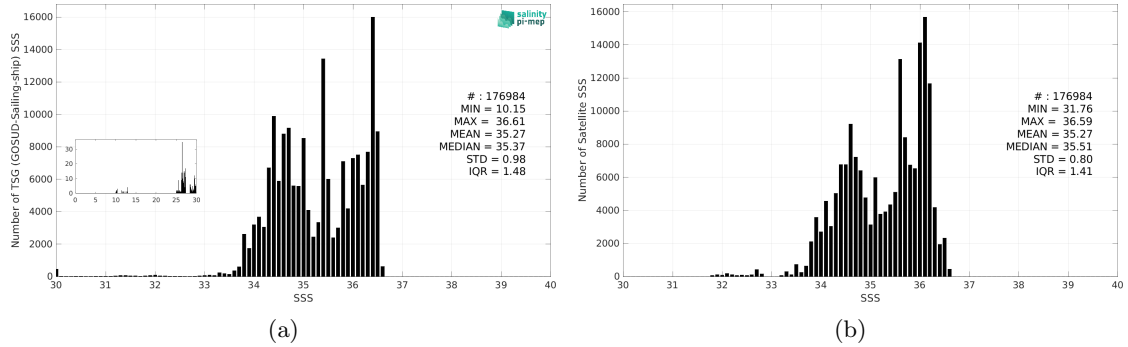
Figure 3: Histograms of SSS from TSG (GOSUD-Sailing-ship) (a) and SMOS SSS L4 v2 - Daily (BEC) (b) considering all match-up pairs per bins of 0.1 over the South Pacific Ocean Pi-MEP region and for the full satellite product period.
