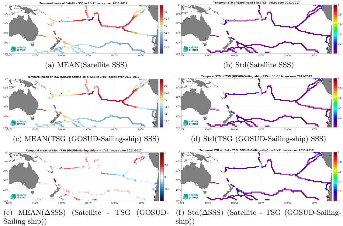
Figure 7: Temporal mean (left) and Std (right) of SSS from SMOS SSS L4 v2 - Daily (BEC) (top), TSG (GOSUD-Sailing-ship) (middle), and of \Delta SSS (Satellite - TSG (GOSUD-Sailing-ship)). Only match-up pairs are used to generate these maps.
