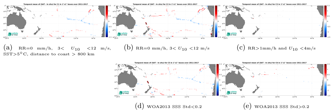
Figure 14: Temporal mean gridded over spatial boxes of size 1^\circ \times 1^\circ of \Delta SSS (SMOS SSS L4 v2 - Daily (BEC) - TSG (GOSUD-Sailing-ship)) for 5 different subdatasets corresponding to:RR=0 mm/h, 3 < U_{10} < 12 m/s, SST>5°C, distance to coast > 800 km (a), RR=0 mm/h, 3 < U_{10} < 12 m/s (b), RR>1mm/h and U_{10} < 4 m/s (c), WOA2013 SSS Std<0.2 (d), WOA2013 SSS Std>0.2 (e).
