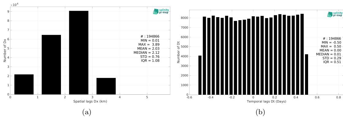
Figure 5: Histograms of the spatial (a) and temporal (b) lags between the location/time of the TSG (GOSUD-Sailing-ship) measurement and the date of the corresponding SMOS SSS L4 v2 - Daily (BEC) SSS pixel.
