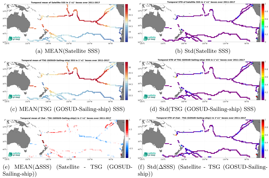
Figure 6: Temporal mean (left) and Std (right) of SSS from SMOS SSS L4 v2 - Daily (BEC) (top), TSG (GOSUD-Sailing-ship) (middle), and of \Delta SSS (Satellite - TSG (GOSUD-Sailing-ship)). Only match-up pairs are used to generate these maps.
