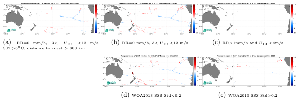
Figure 12: Temporal mean gridded over spatial boxes of size 1^\circ \times 1^\circ of \Delta SSS (SMOS SSS L4 v2 - Daily (BEC) - TSG (GOSUD-Sailing-ship)) for 5 different subdatasets corresponding to:RR=0 mm/h, 3 < U_{10} < 12 m/s, SST>5°C, distance to coast > 800 km (a), RR=0 mm/h, 3 < U_{10} < 12 m/s (b), RR>1mm/h and U_{10} < 4 m/s (c), WOA2013 SSS Std<0.2 (d), WOA2013 SSS Std>0.2 (e).
