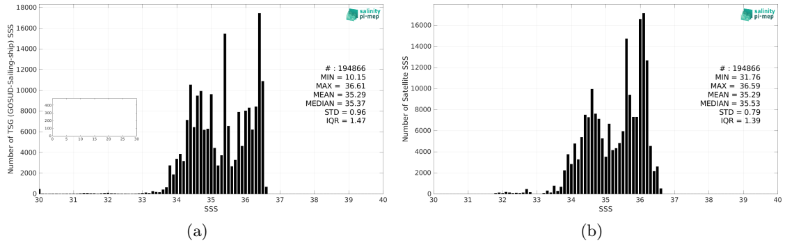
Figure 2: Histograms of SSS from TSG (GOSUD-Sailing-ship) (a) and SMOS SSS L4 v2 - Daily (BEC) (b) considering all match-up pairs per bins of 0.1 over the South Pacific Ocean Pi-MEP region and for the full satellite product period.
