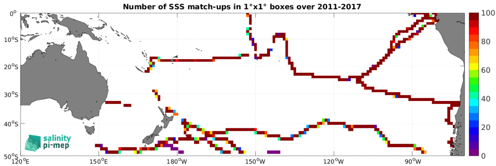
Figure 4: Number of SSS match-ups between TSG (GOSUD-Sailing-ship) SSS and the SMOS SSS L4 v2 - Daily (BEC) SSS product for the South Pacific Ocean Pi-MEP region over 1^\circ \times 1^\circ boxes and for the full satellite product period.
