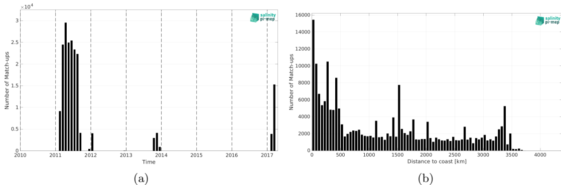
Figure 1: Number of match-ups between TSG (GOSUD-Sailing-ship) and SMOS SSS L4 v2 - Daily (BEC) SSS as a function of time (a) and as function of the distance to coast (b) over the South Pacific Ocean Pi-MEP region and for the full satellite product period.
