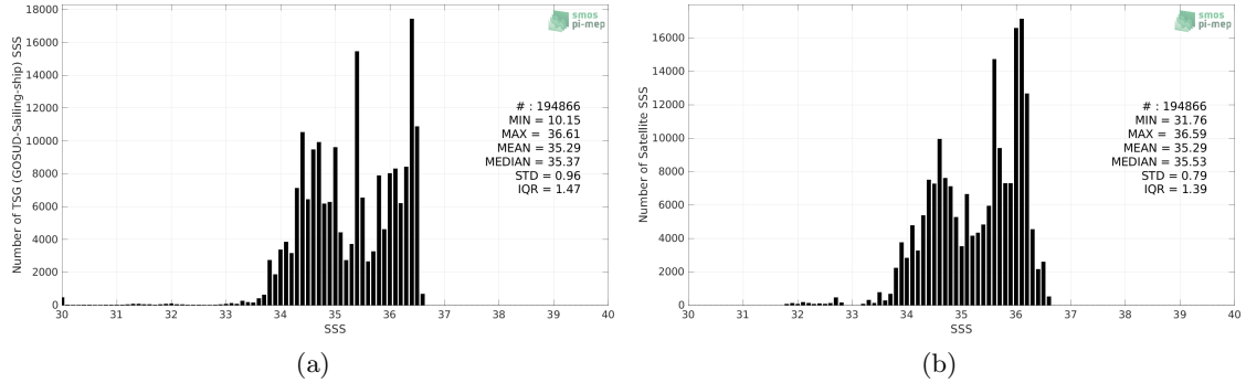
Figure 2: Histograms of SSS from TSG (GOSUD-Sailing-ship) (a) and SMOS SSS L4 v2 - Daily (BEC) (b) considering all match-up pairs per bins of 0.1 over the South Pacific Ocean Pi-MEP region and for the full satellite product period.
