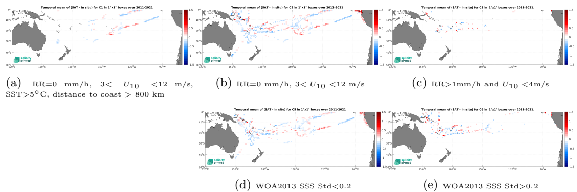
Figure 14: Temporal mean gridded over spatial boxes of size 1^\circ \times 1^\circ of \Delta SSS (SMOS SSS L4 v2 - Daily (BEC) - TSG (GOSUD-Research-vessel)) for 5 different subdatasets corresponding to:RR=0 mm/h, 3 < U_{10} < 12 m/s, SST >5^\circ\text{C} , distance to coast > 800 km (a), RR=0 mm/h, 3 < U_{10} < 12 m/s (b), RR >1 mm/h and U_{10} < 4 m/s (c), WOA2013 SSS Std <0.2 (d), WOA2013 SSS Std >0.2 (e).
