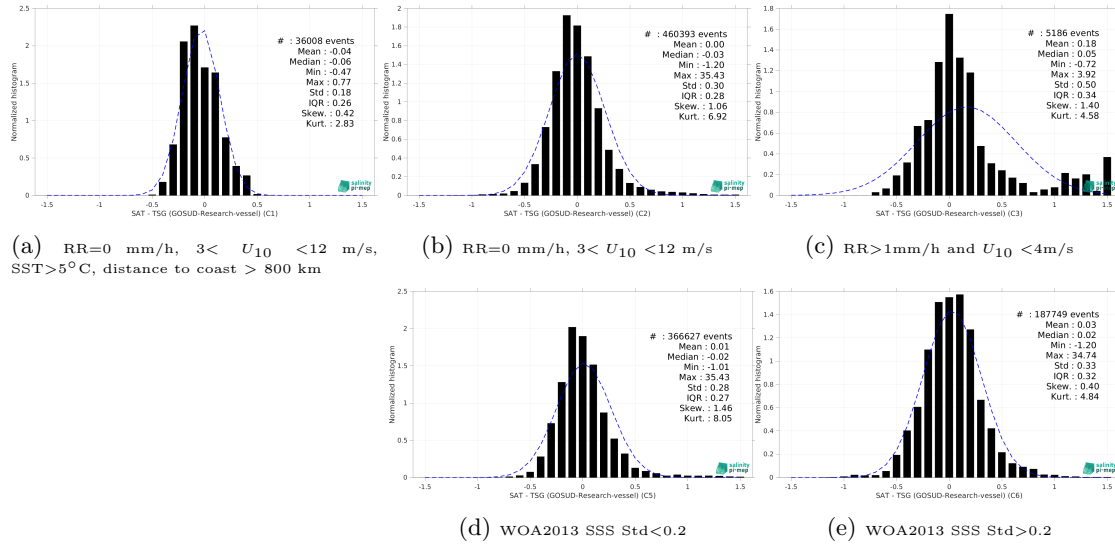
Figure 15: Normalized histogram of \Delta\text{SSS} (SMOS SSS L4 v2 - Daily (BEC) - TSG (GOSUD-Research-vessel)) for 5 different subdatasets corresponding to: RR=0 mm/h, 3 < U_{10} < 12 m/s, SST>5°C, distance to coast > 800 km (a), RR=0 mm/h, 3 < U_{10} < 12 m/s (b), RR>1mm/h and U_{10} < 4 m/s (c), WOA2013 SSS Std<0.2 (d), WOA2013 SSS Std>0.2 (e).
